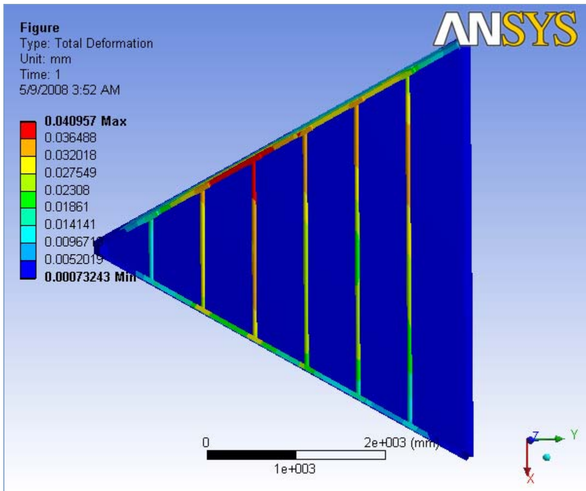
FIGURE 11 Orientation 4.1 refined > Static Structural > Solution > X - Directional Deformation > Figure
