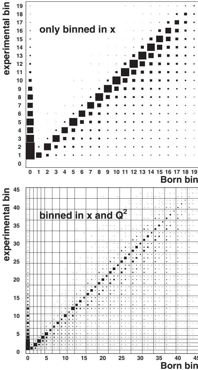
FIG. 17. Migration matrices M_{\vec{z}} (the M_{\vec{z}} matrices look similar) for two different binnings. Top panel: migration matrix for a pure x binning. Bottom panel: migration matrix for the combined x and Q^2 binning used in this analysis. The horizontal and vertical lines divide the x bins; within each x bin the Q^2 bins are arranged in increasing Q^2 . The matrices are extracted from a fully reconstructed Monte Carlo data set simulating both QED radiative and detector effects for inclusive DIS on a proton target.
