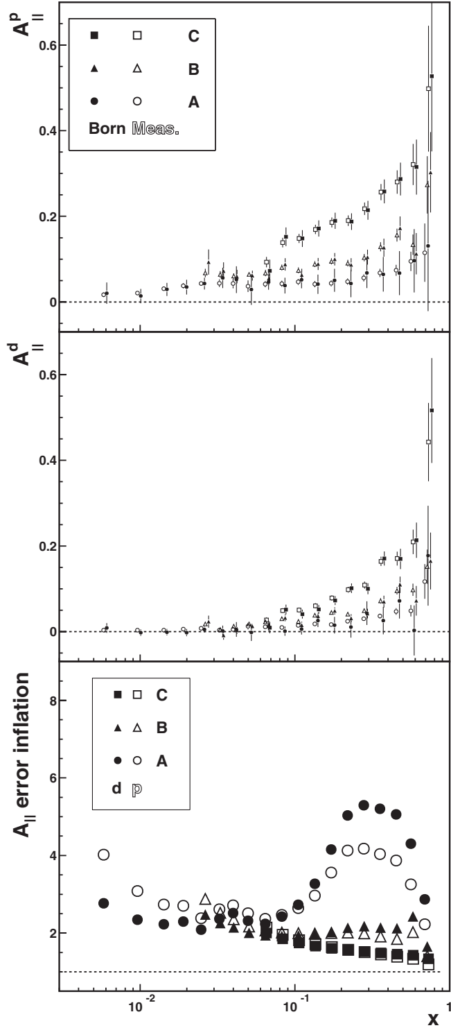
FIG. 18. Top two panels: measured and unfolded Born asymmetries for the proton and deuteron. The error bars of the Born asymmetries are the square root of the diagonal elements of the covariance matrix obtained after unfolding, with the inclusion of the uncertainty due to the statistics of the Monte Carlo. Bottom panel: uncertainty inflation when going from measured to Born asymmetry due to the unfolding procedure. The symbols A, B, and C refer to the Q^2 -bin sets defined in Fig. 4.
