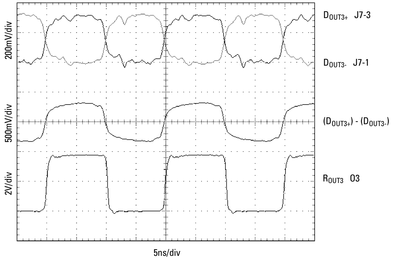
LVDS Channel #3 Waveforms - 5m Cable Interconnect
