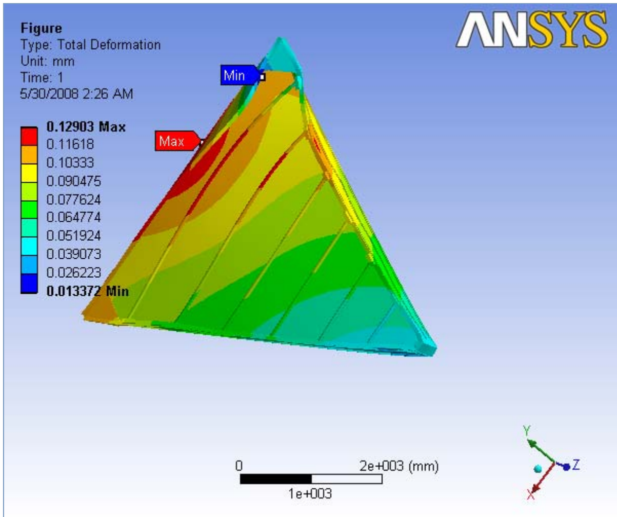
FIGURE 11 sector 1, Case 4 > Static Structural > Solution > X - Directional Deformation > Figure
