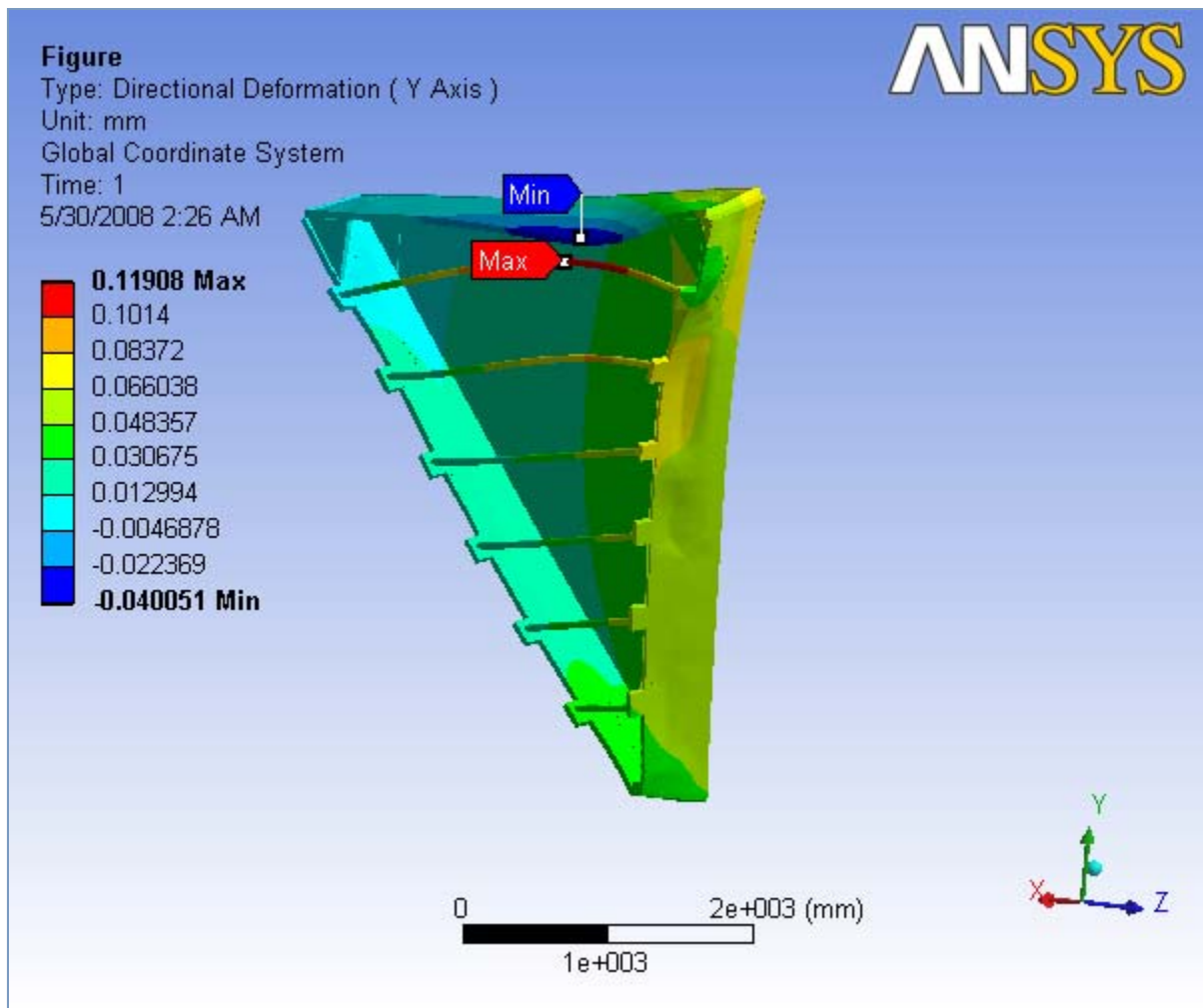
FIGURE 13 sector 1, Case 4 > Static Structural > Solution > Z - Directional Deformation > Figure
