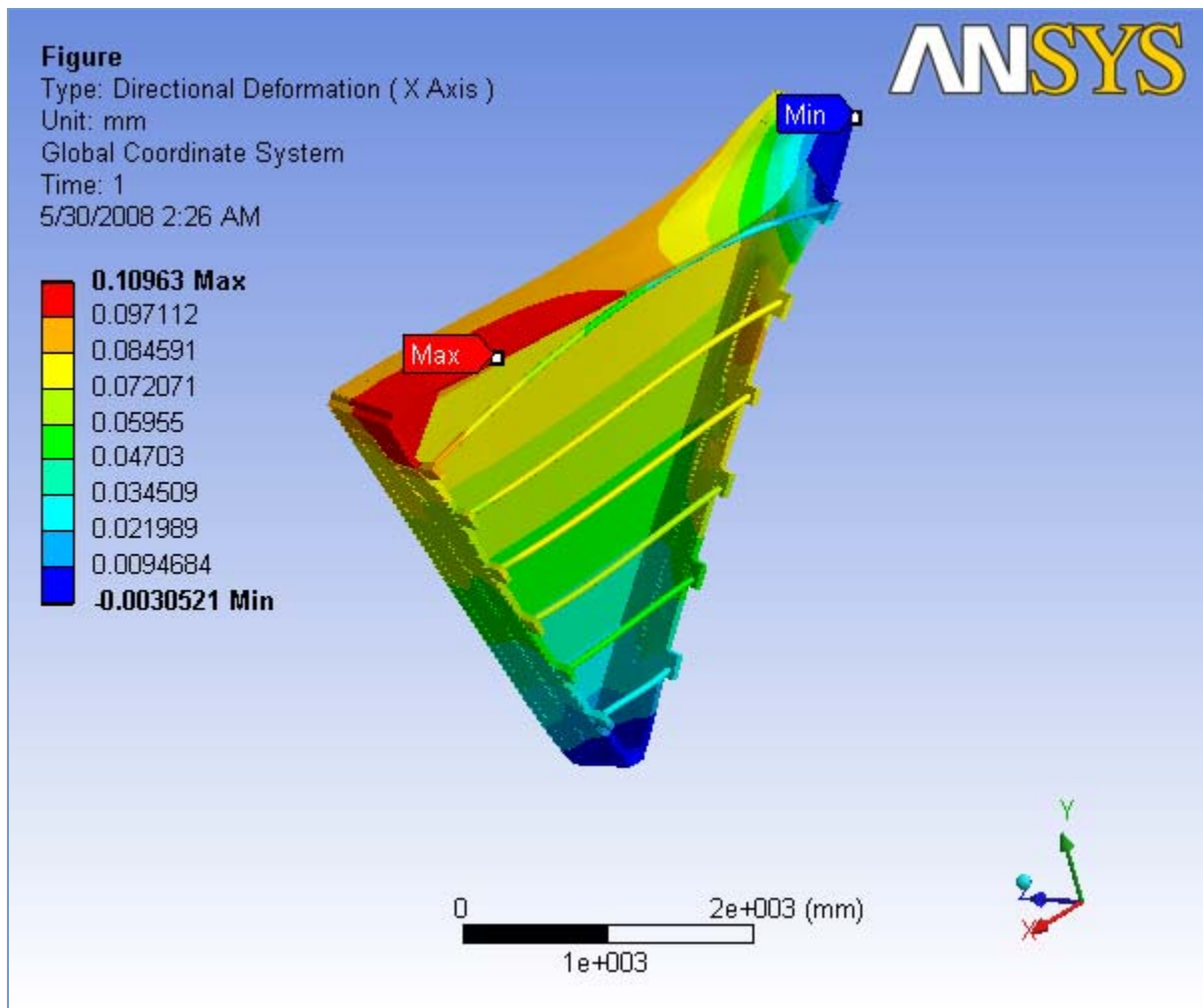
FIGURE 12 sector 1, Case 4 > Static Structural > Solution > Y - Directional Deformation > Figure
