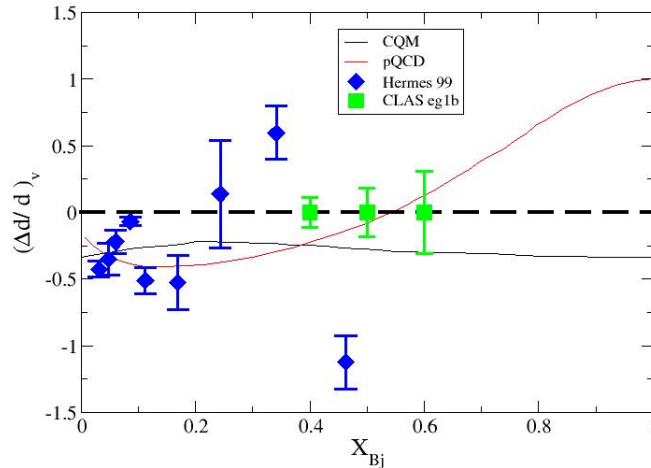
Figure 9. The ratio of polarized to unpolarized valence down quark distribution function vs x_{Bj} [20] .
