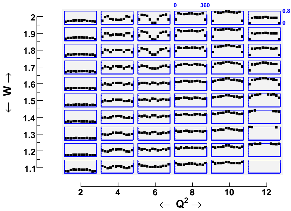
Figure 34: \phi_\pi evolution of the \pi^+ acceptance in the forward \cos\theta_\pi = 0.1 \pm 0.1 bin for the resonance region and the proposed Q^2 range.
