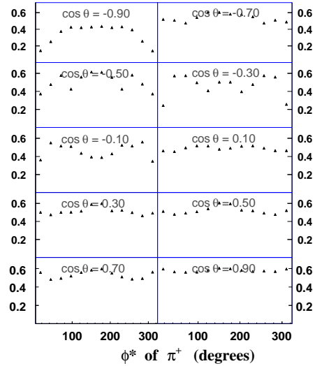
Figure 35: \phi_\pi evolution of the \pi^+ acceptance in a specific W and Q^2 bin for the full \cos\theta_\pi range.
