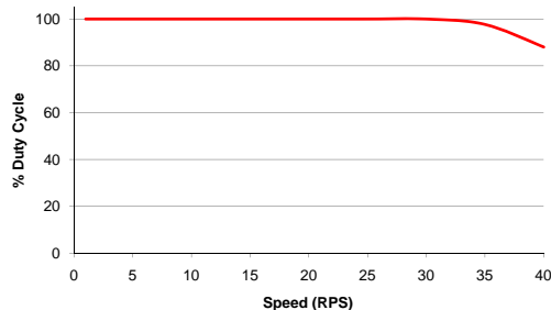
HT34-487 Max Duty Cycle vs Speed 24VDC, 8A parallel 40 °C Ambient on a 10 x 10 x .5 Aluminum Plate
