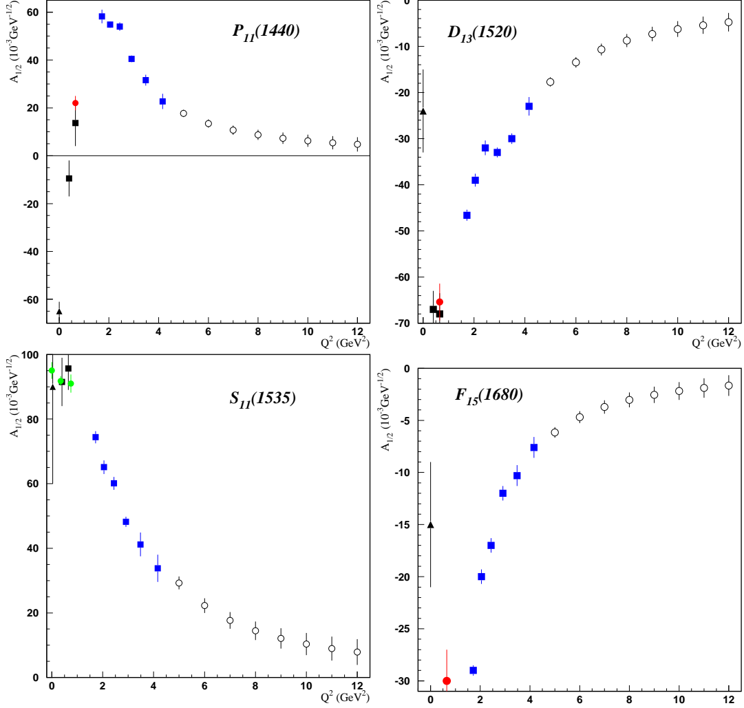
Figure 41: Projected N^* electrocoupling amplitudes as expected from our proposed experiment (open circles with error bars). Also shown are the electrocoupling amplitudes extracted from the available CLAS data on 1\pi electroproduction [?] (black filled squares), data from analysis of e1-6 run [47] (blue filled squares), and the results from a combined analysis of the 1\pi and 2\pi electroproduction channels [67].
