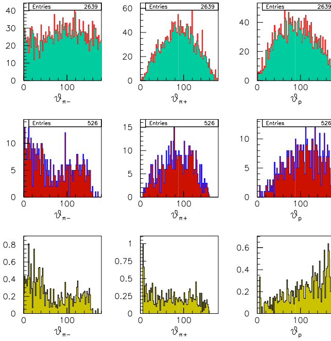
Figure 33: Efficiency for various angular distributions in 2\pi production averaged over the four other kinematics variables at W from 1.5 to 1.7 GeV and at Q^2 from 5.0 to 10.0 \text{GeV}^2 . The distributions for generated and accepted events are shown in the top and middle row, respectively. The estimated efficiencies are presented in the bottom row.
