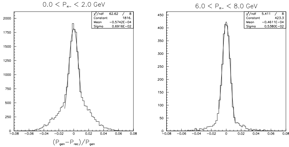
Figure 34: Momentum resolution for \pi^- . p_{rec} and p_{gen} represent the momentum for reconstructed and generated particles, respectively.
