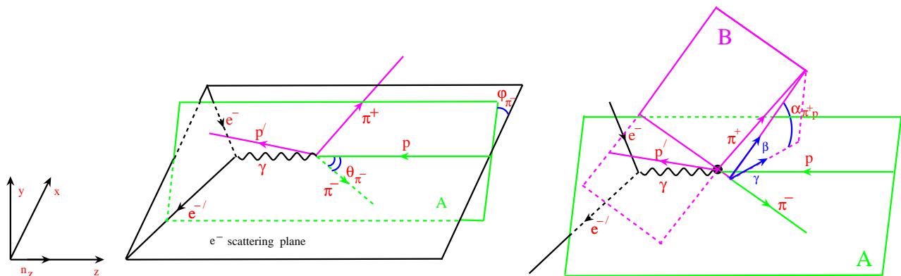
Figure 27: Angular variables used in the analysis of the 2\pi production CLAS data.
