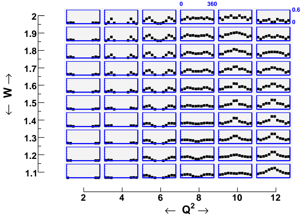
Figure 22: \phi_\pi evolution of the \pi^0 acceptance in the forward \cos\theta_\pi = 0.1 \pm 0.1 bin for the resonance region and the proposed Q^2 range.
