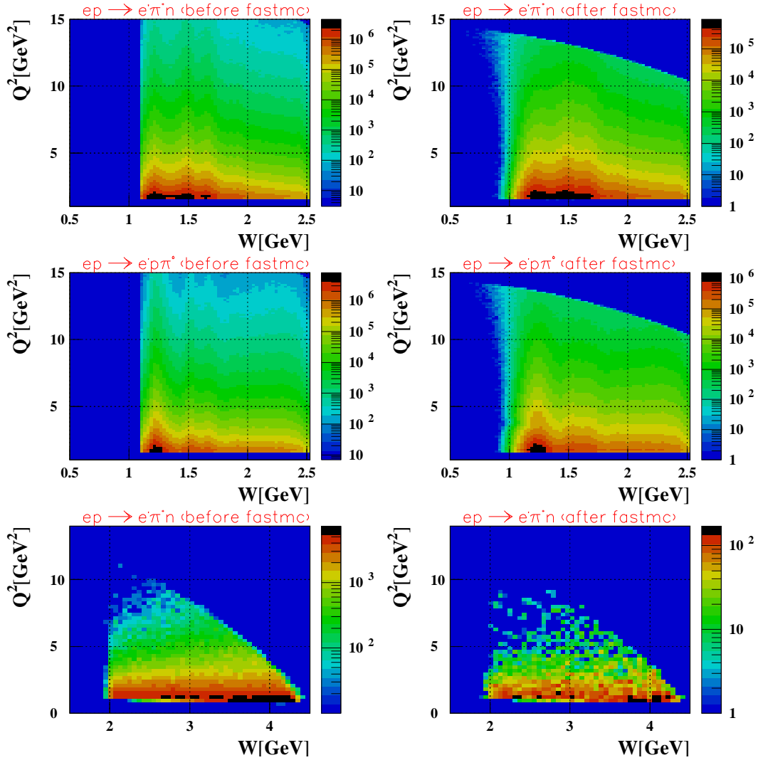
Figure 18: Kinematic coverage of CLAS12 in the resonance region for the exclusive one pion electro-production at 11\text{ GeV} electron beam energy when e' and \pi^+ (upper and lower right panels) or e' and p (middle right panel) are detected in the CLAS12 FastMC simulation based on the Genova-EG (in the resonance region) or DIS (beyond the resonance region) event generator, and the corresponding Genova-EG (upper and middle left panels) and DIS (lower left panel) event generator data itself.
