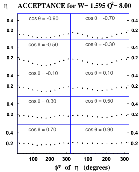
Figure 25: \phi_\eta evolution of the \eta acceptance in a specific W and Q^2 bin for the full \cos\theta_\eta range.
