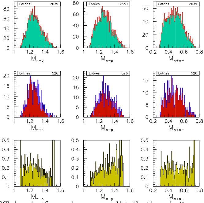
Figure 32: Efficiencies for various mass distributions in 2\pi production averaged over W from 1.5 to 1.7 GeV and Q^2 from 5.0 to 10.0 \text{GeV}^2 . The distributions for generated and accepted events are shown in the top and middle rows, respectively. The estimated efficiencies are presented in the bottom row.
