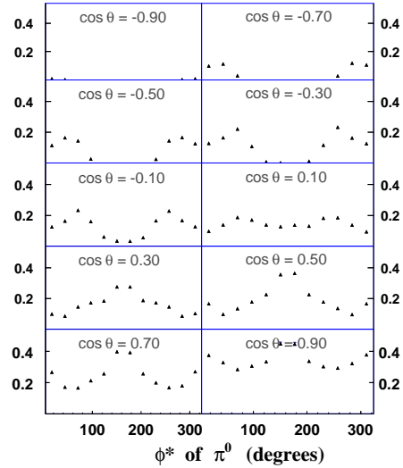
Figure 23: \phi_\pi evolution of the \pi^0 acceptance in a specific W and Q^2 bin for the full \cos\theta_\pi range.
