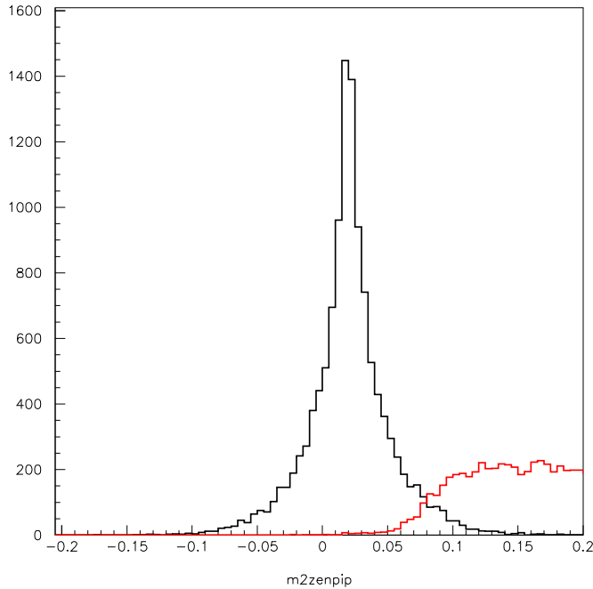
Figure 29: Distributions of M_{\pi^+ p_X}^2 for detected 2\pi (black) and 3\pi events (red) curves.
