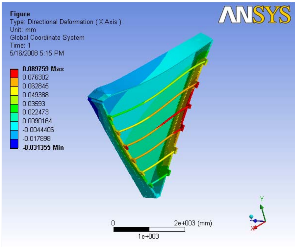
FIGURE 12 Sector 2 > Static Structural > Solution > Y - Directional Deformation > Figure
