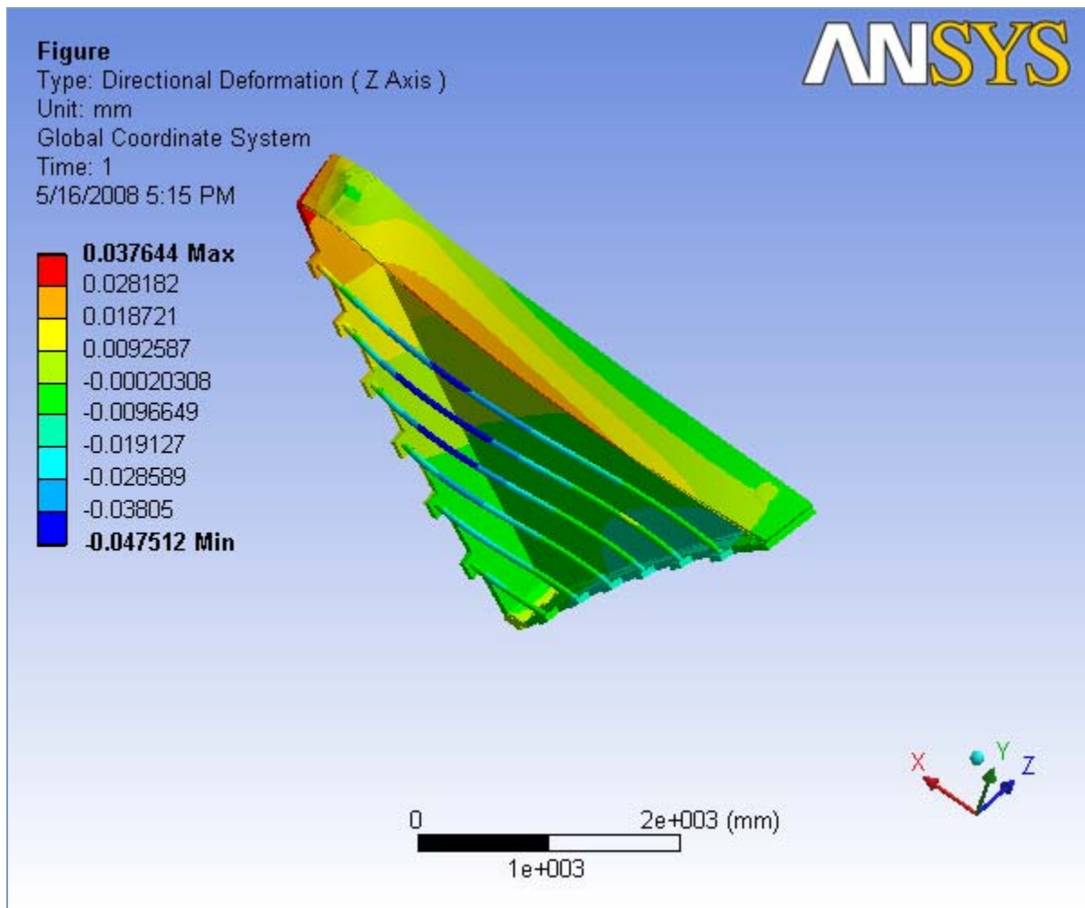
FIGURE 14 Sector 2 > Static Structural > Solution > Equivalent Stress > Figure
