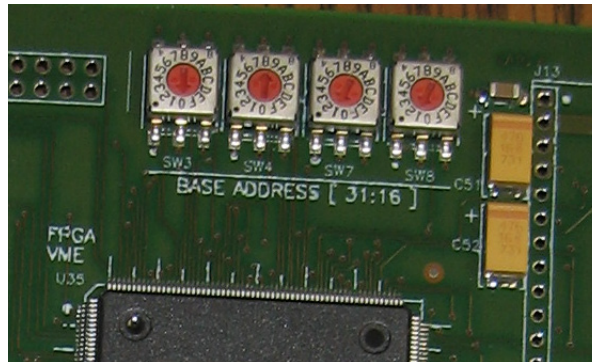
Figure 1-1: Hexidecimal Address Switches on V1495
