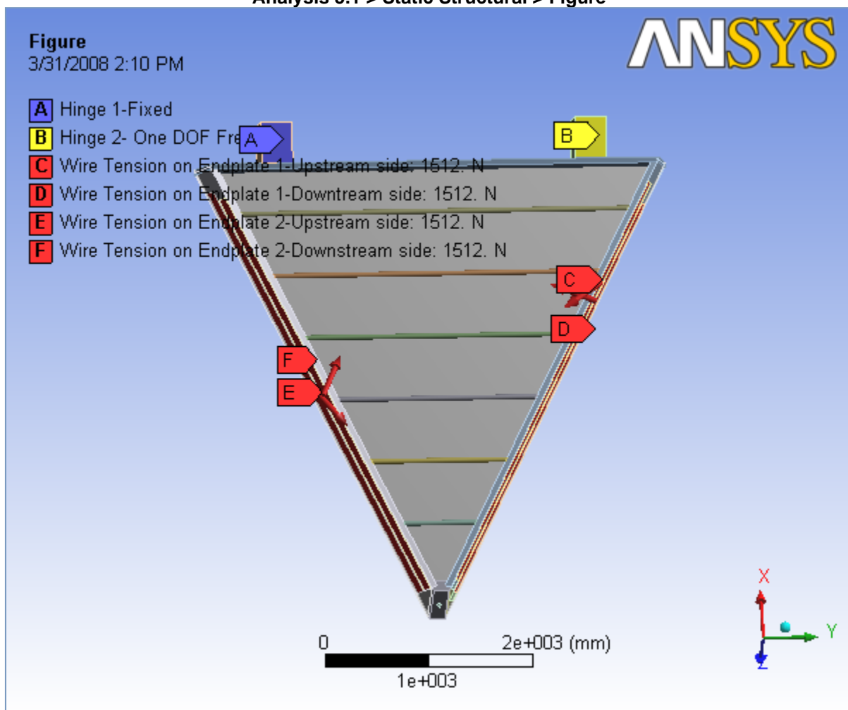
FIGURE 1 Analysis 5.1 > Static Structural > Figure
