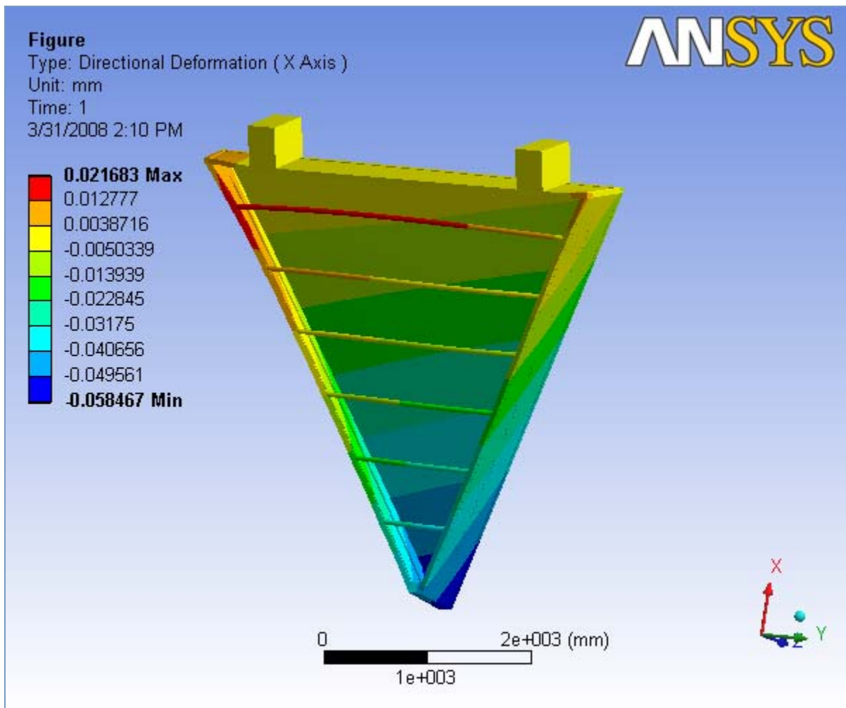
FIGURE 10 Analysis 5.1 > Static Structural > Solution > y Directional Deformation > Figure
