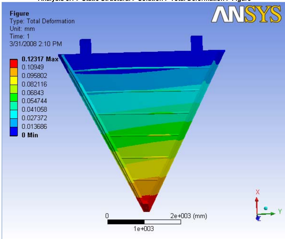
FIGURE 8 Analysis 5.1 > Static Structural > Solution > Total Deformation > Figure
