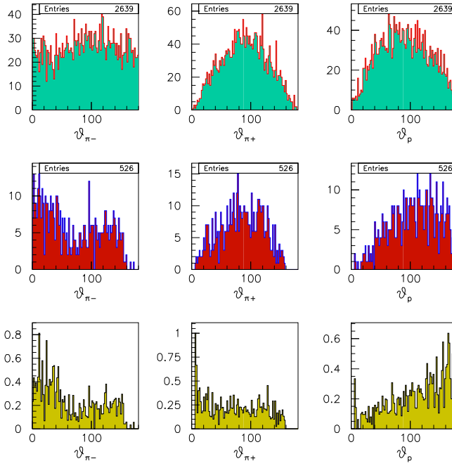
Figure 32: Efficiency for various angular distributions in 2\pi production averaged over the four other kinematics variables at W from 1.5 to 1.7 GeV and at Q^2 from 5.0 to 10.0 \text{GeV}^2 . The distributions for generated and accepted events are shown in the top and middle row, respectively. The estimated efficiencies are presented in the bottom row.
