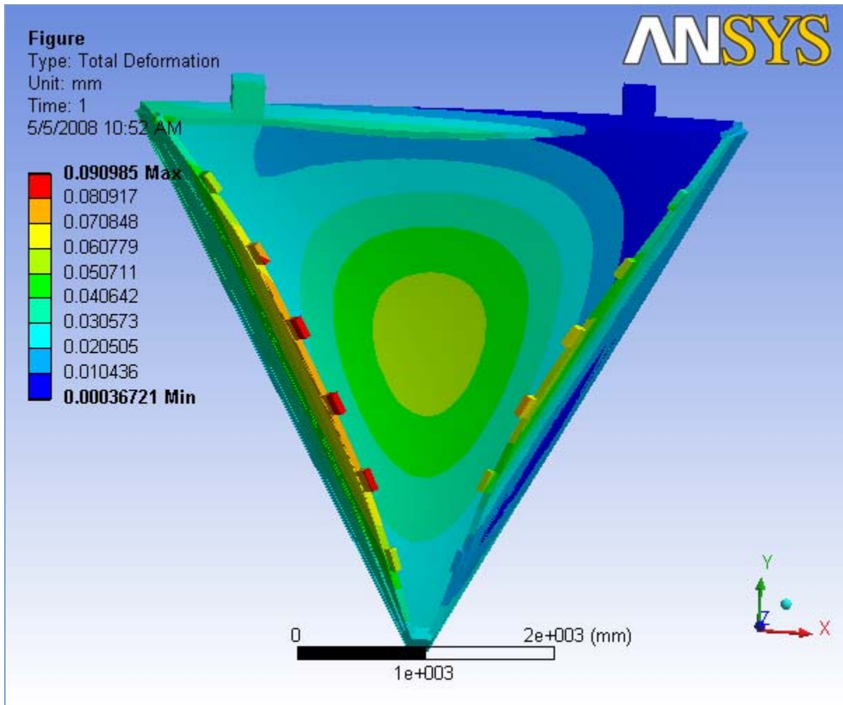
FIGURE 11 Ideal slice with Wire loads, Hexcel, Gravity (No Rods) > Static Structural > Solution > X - Directional Deformation > Figure
