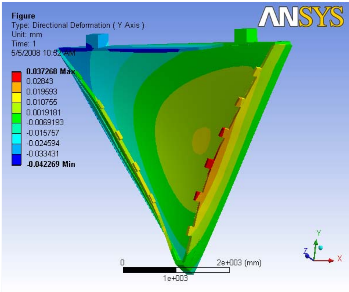
FIGURE 13 Ideal slice with Wire loads, Hexcel, Gravity (No Rods) > Static Structural > Solution > Z - Directional Deformation > Figure
