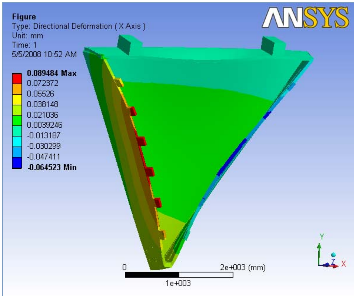
FIGURE 12 Ideal slice with Wire loads, Hexcel, Gravity (No Rods) > Static Structural > Solution > Y - Directional Deformation > Figure
