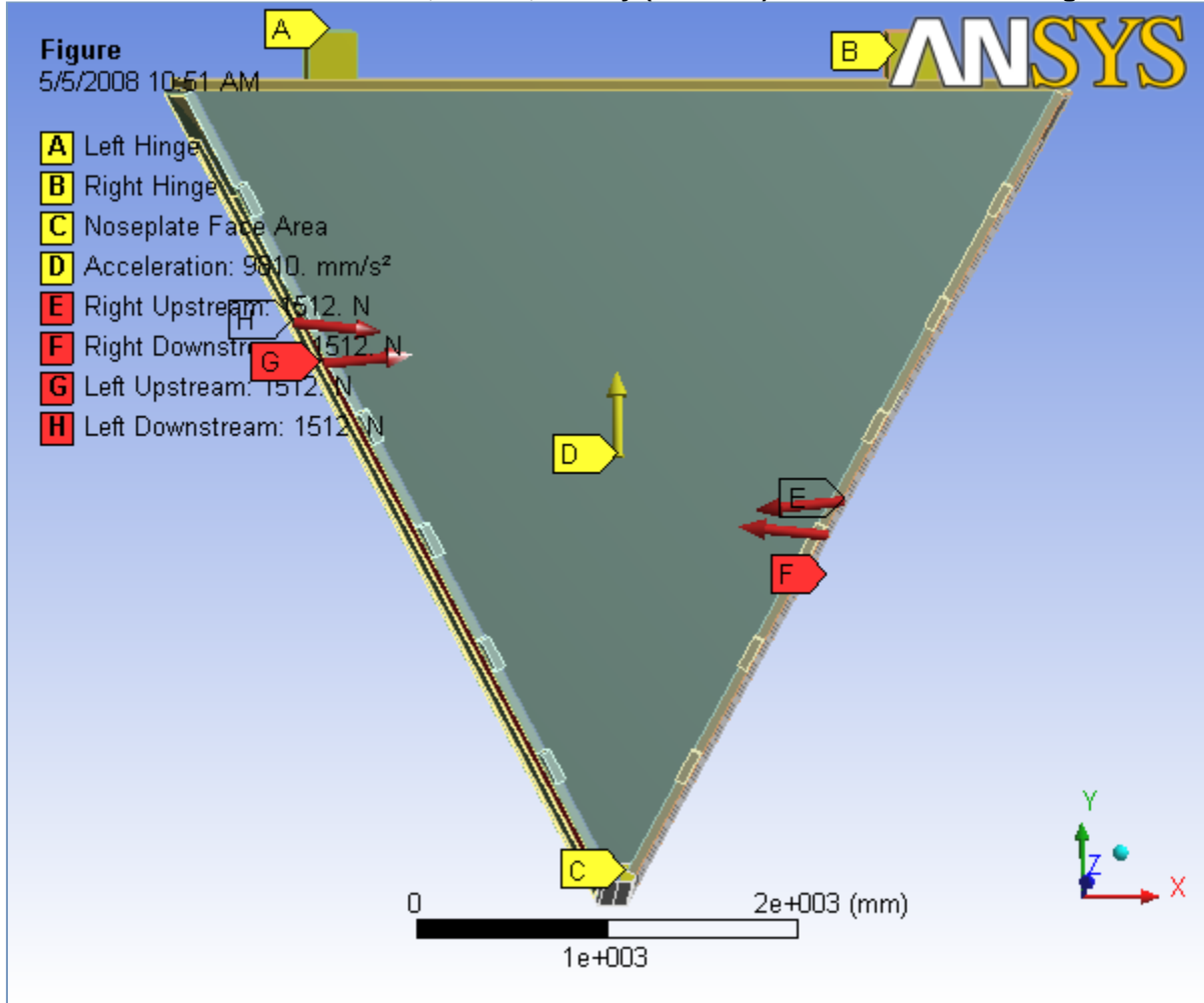
FIGURE 1 Ideal slice with Wire loads, Hexcel, Gravity (No Rods) > Static Structural > Figure
