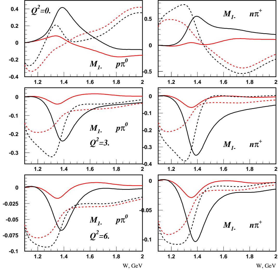
Figure 9: The M_{1-} multipole amplitude for the reactions \gamma^* p \rightarrow p\pi^0 (left) and n\pi^+ (right) at Q^2 = 0, 3, \text{ and } 6 \text{GeV}^2 . Black curves are the total amplitudes, red curves represent the background; each separated into imaginary (real) part and represented by solid (dashed) curves.
