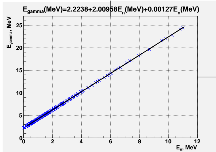
Figure 25: Correlation plot for neutron energies and photon energies. Neutrons are coming from D_2 only.
