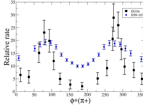
Figure 8. \varphi_{\pi^*} vs Relative rate for fixed \cos\theta_{pion}^{CM} = 0.5 and W = 1.45\text{GeV} [18], [19].
