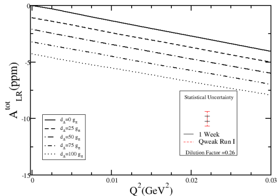
Figure 6: The expected statistical uncertainty for a measurement of d_\Delta using the current data set from the last Qweak run and assuming a full week of beam time.
