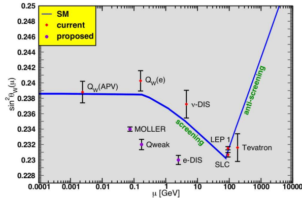
Figure 5: The dependence of \sin^2\theta_W on Q^2 cast in the \overline{MS} scheme of reference [17]. The three future measurements are located at appropriate \mu values but the vertical locations are arbitrary.
