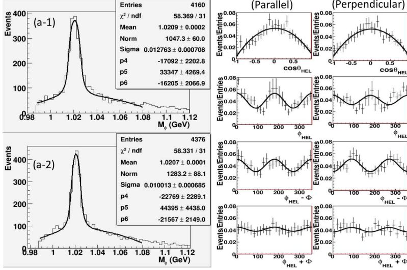
Figure 9: \vec{\gamma}p \rightarrow \phi p and 1.7 < E_\gamma < 1.9 GeV. Left side: \phi -meson distribution fit with a Breit-Wigner convoluted with a Gaussian peak ( \sigma \sim 11 MeV) and a 2 nd order polynomial background. Here, the direction of the polarization vector ( vecE ): (a-1) Parallel and (a-2) Perpendicular to the floor in the CLAS lab frame. Right side: Angular distributions of the \phi -meson in the Helicity frame. First (second) column is for \vec{E}_\parallel ( \vec{E}_\perp ). Of especial interest are the angular distributions as a function of \cos \theta_{Hel} showing the expected \sin^2 \theta_{Hel} -like behavior and the modulation as a function of azimuth ( \phi_{Hel} - \Phi ).
