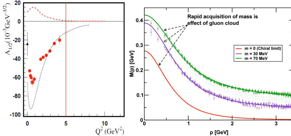
Figure 3: Left side: Electrocouplings for D_{13}(1520) state determined from the CLAS data on N\pi electroproduction [?] (red points) from a combined analysis of the N\pi and N\pi\pi channels. Differences between the data at Q^2 < 1.0 \text{GeV}^2 and quark model [?] calculations (dotted curve) highlight possible contributions from meson-baryon dressing (red dashed curve) [?]. Right side: Dressed quark mass as a function of momentum for light-quarks, obtained in the Landau gauge: solid curves are the Dyson Schwinger Equation results, including the chiral-limit [?, ?]; points with error bars are the results from unquenched LQCD [?].
