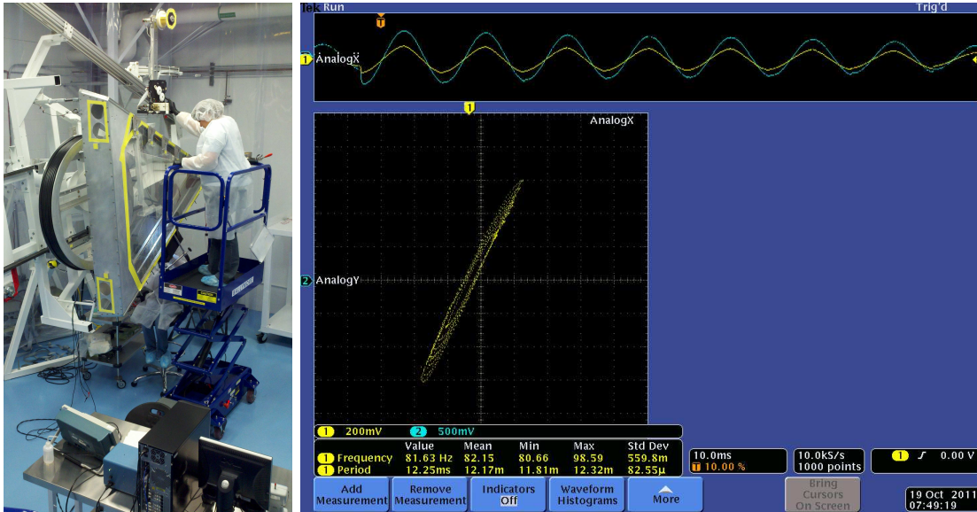
Figure 1: The left figure shows a photograph of two technicians constructing the a R1 drift chamber in the ISU physics clean room. The right figure is an illustration of the signal observed during the wire tension measurements [1].
