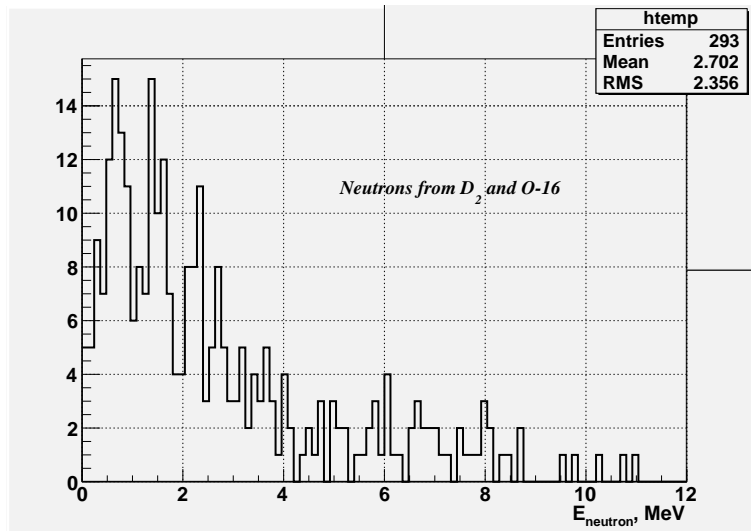
Figure 24: Neutron energy spectrum is the sum of neutrons from D_2 and O - 16 .
