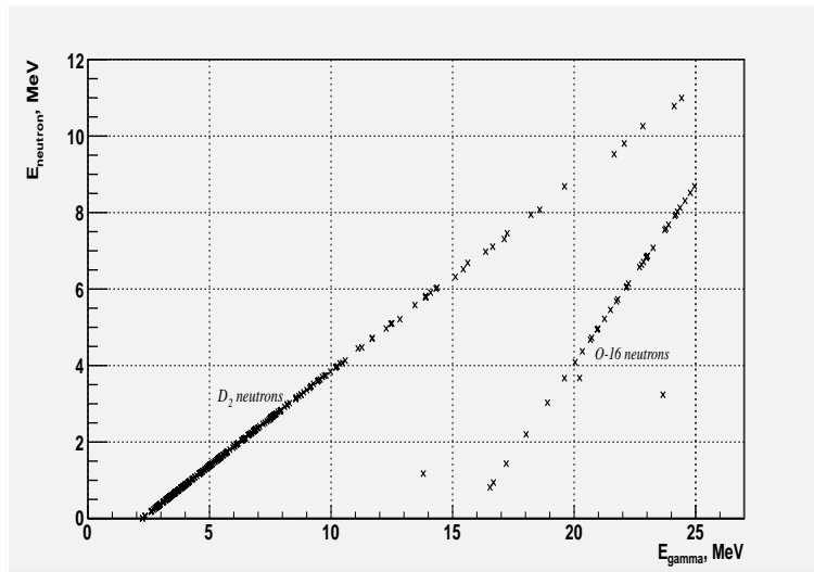
Figure 22: Correlation plot.
