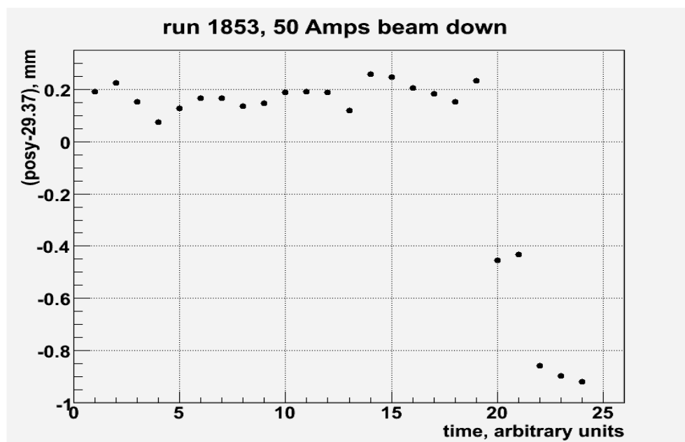
Temporal variation of beam in Y-direction for different kicker magnet currents. (time increment 1000 events)
