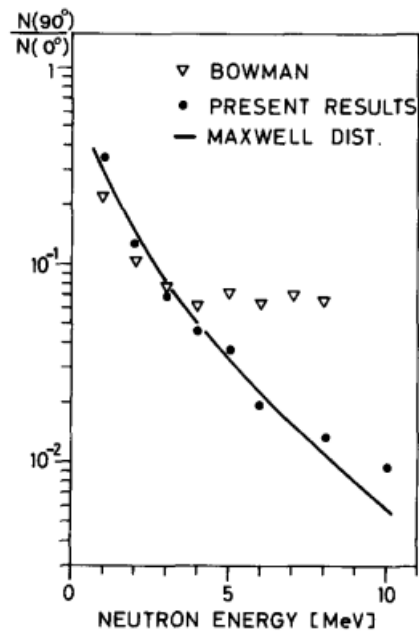
Figure 2.6: Fission neutron intensity ratio N(90^\circ)/N(0^\circ) is plotted versus the fission neutron energy. The full line represents this ratio calculated with the assumption of neutron evaporation from the fully accelerated fragments.
