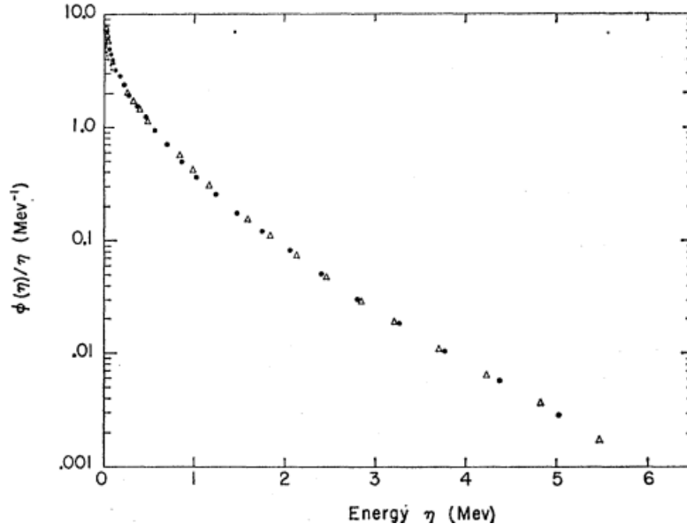
Figure 2.3: The center-of-mass neutron energy spectrum \phi(\eta) (c.m) divided by \eta .
