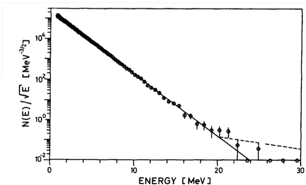
Figure 2.4: Fission neutron energy spectrum divided by the square root of the neutron energy versus the neutron energy. The solid line is Maxwell energy distribution.
