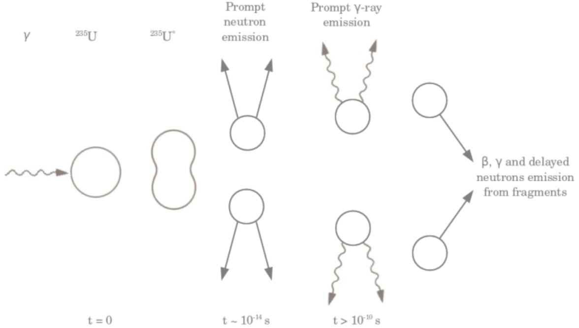
Figure 1.1: Schematic representation of the fission process in uranium. Neutrons are emitted after while from fully accelerated fission fragments. The times scale gives the orders of magnitude only.
