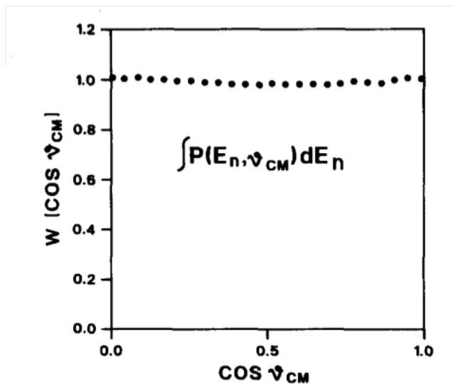
Figure 2.5: Fission neutron angular distribution in the fragment center-of-mass system integrated over all neutron energies
