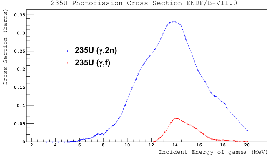
Figure 4.5: ^{235}\text{U} photofission cross section taken from ENDF/B-VII.0
