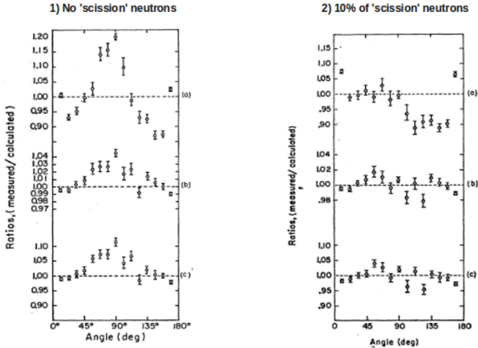
Figure 2.2: The ratio of measured to calculated values for (a) numbers of neutrons (b) average velocities, and (c) average energies as a function of angles. (1) In the left picture the calculated values were obtained by using a three-temperature- evaporation formula. (2) In the right picture 10% of the total number of neutrons are assumed to come from scission (not evaporated from the fragments).
