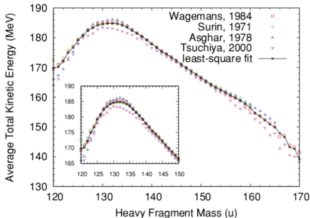
Figure 1.2: The average TKE as a function of the heavy fragment mass. The solid line is the resulting of a least-square fitting of the experimental data sets
