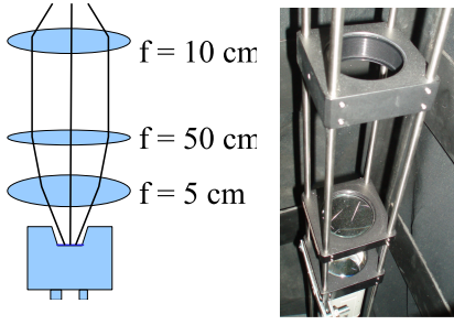
Figure 2: The OTR Imaging system.
