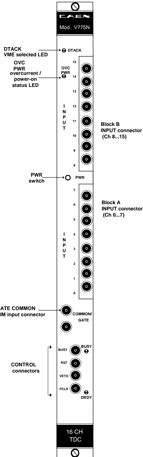
Fig. 3.2: Model V775 N front panel
