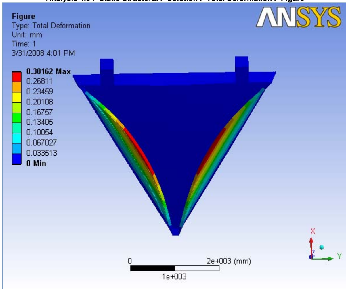
FIGURE 8 Analysis 4.3 > Static Structural > Solution > Total Deformation > Figure
