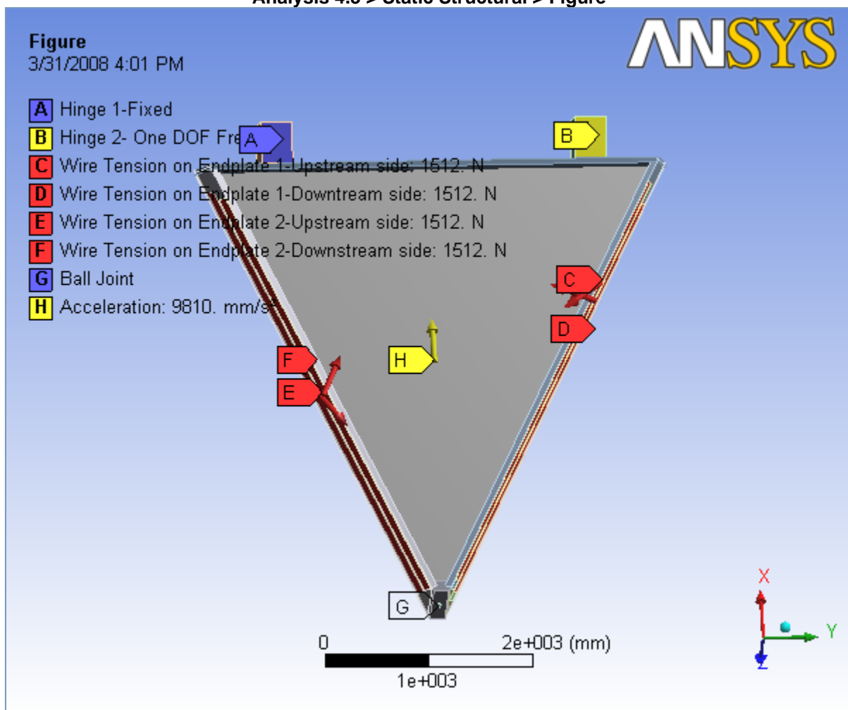
FIGURE 1 Analysis 4.3 > Static Structural > Figure
