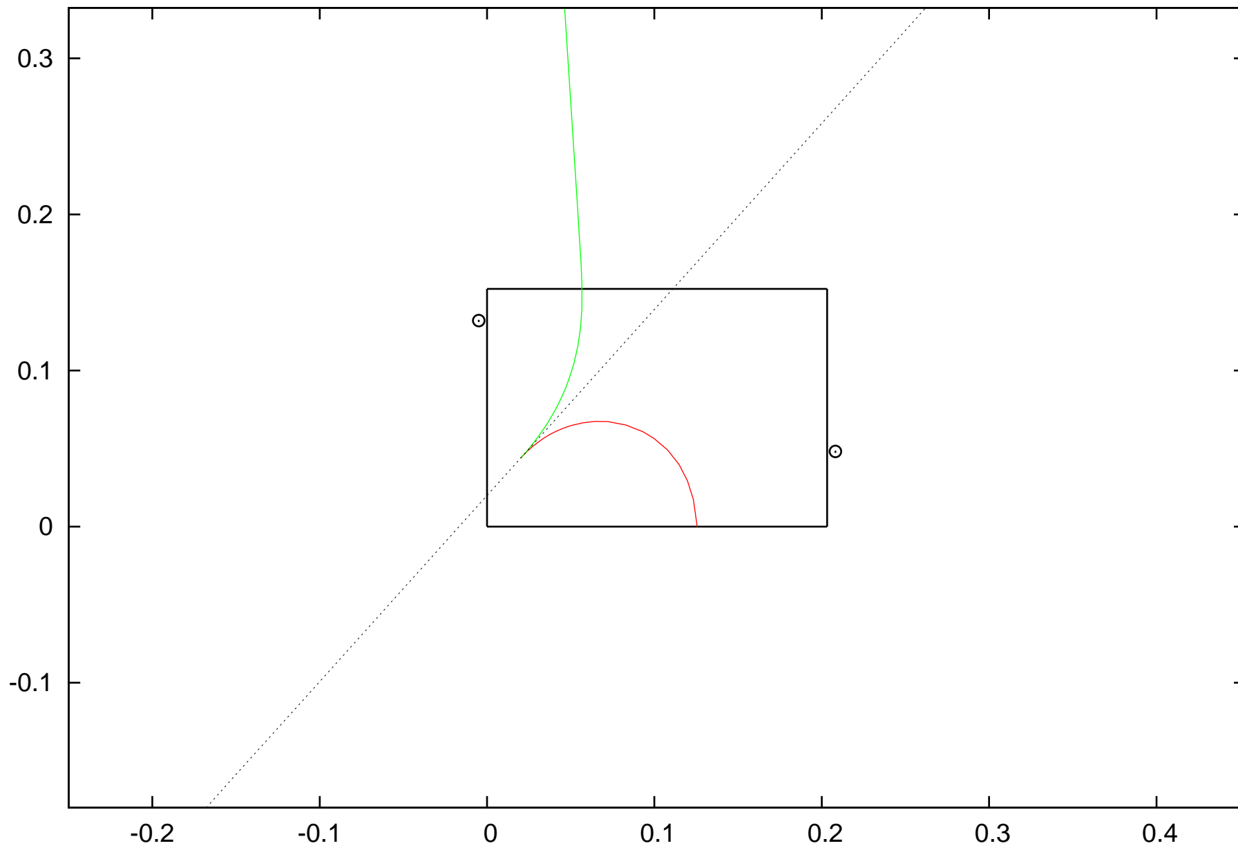
Electron energy: 1.5 MeV, Conversion at (0.02,0.0438351)
