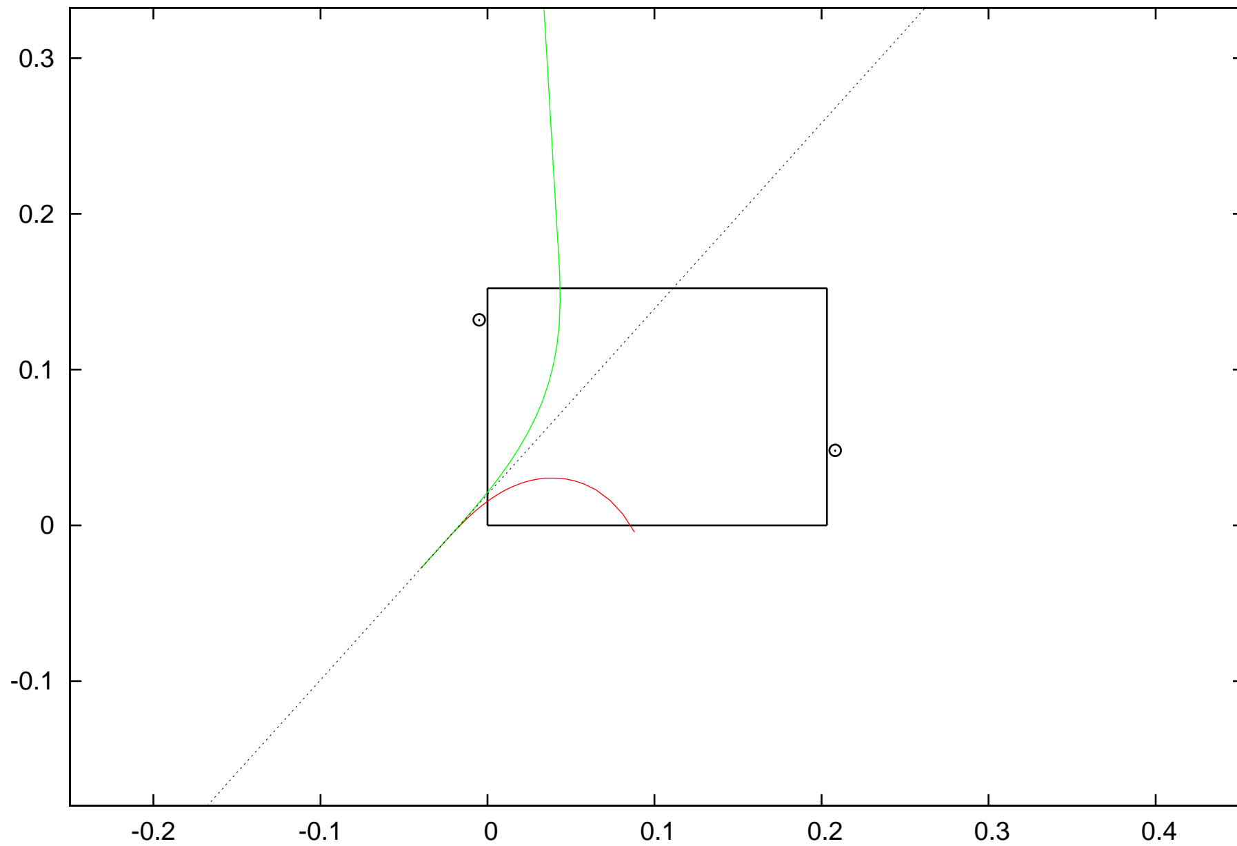
Electron energy: 1.0 MeV, Conversion at (-0.04,-0.0276701)
