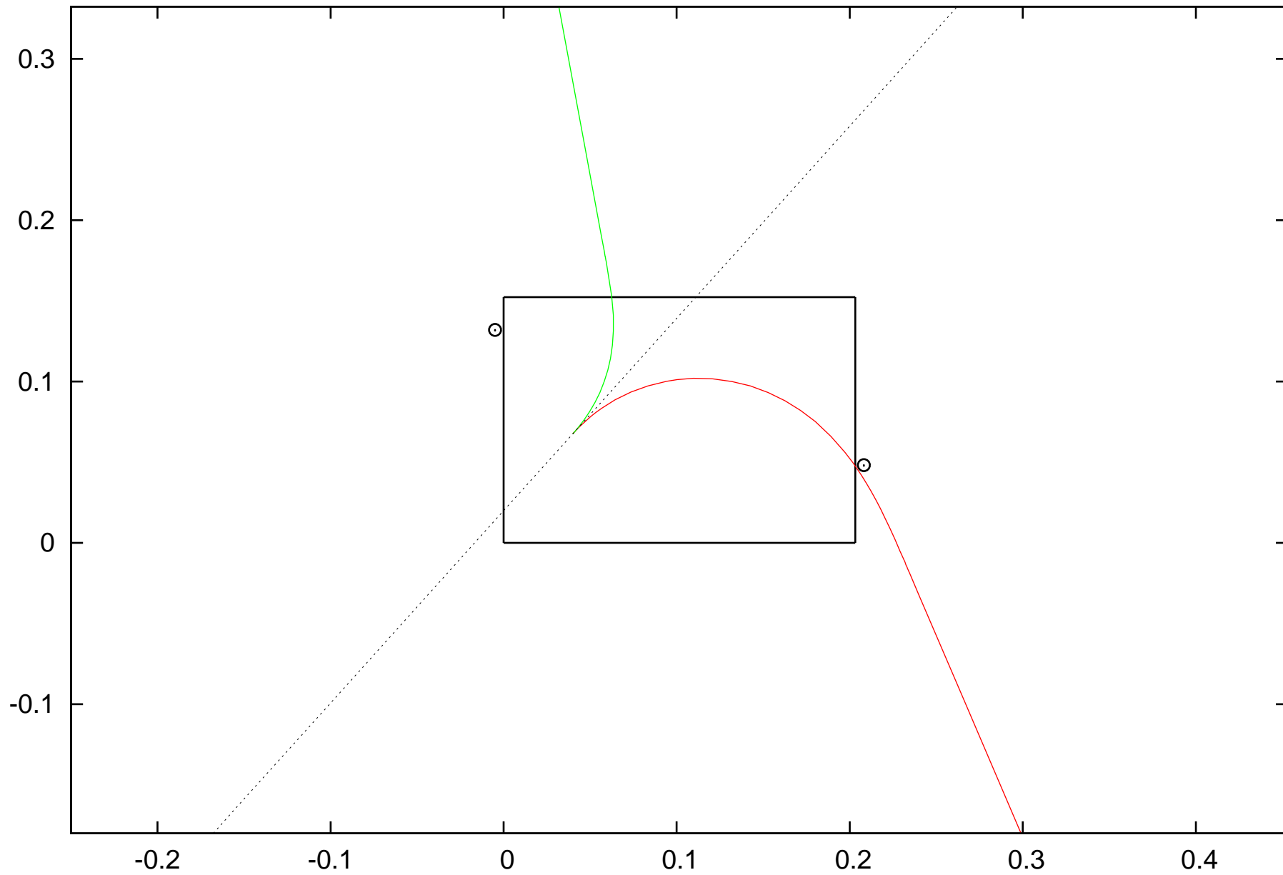
Electron energy: 2.5 MeV, Conversion at (0.04,0.0676701)
