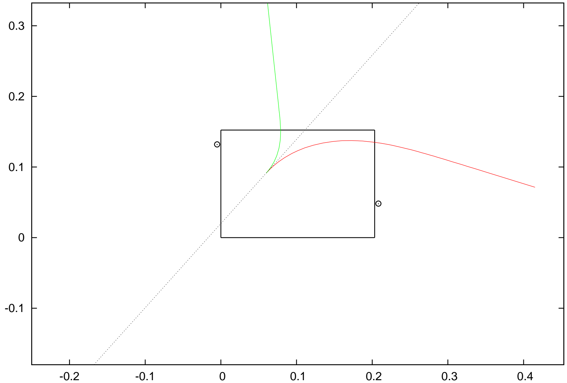
Electron energy: 3.0 MeV, Conversion at (0.06,0.0915052)
