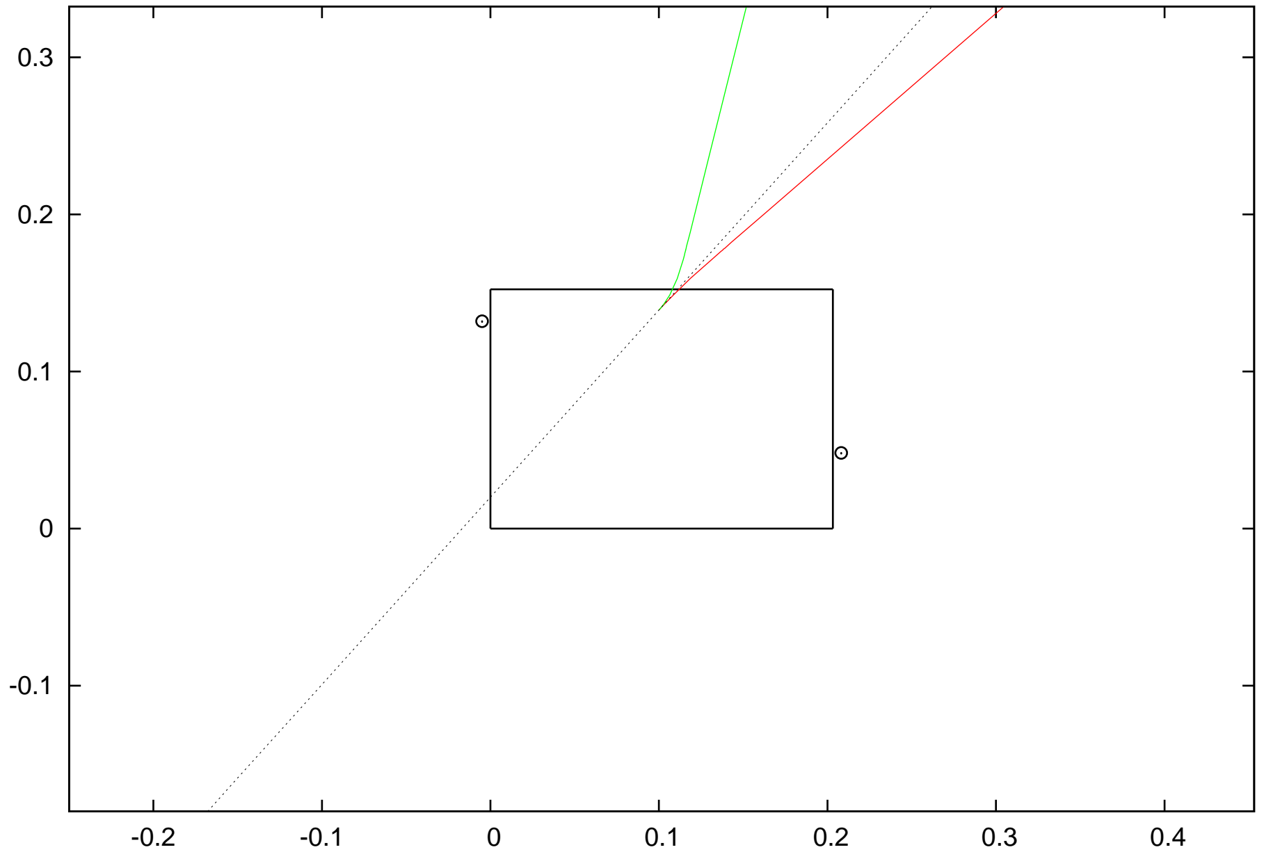
Electron energy: 4.0 MeV, Conversion at (0.1,0.139175)
