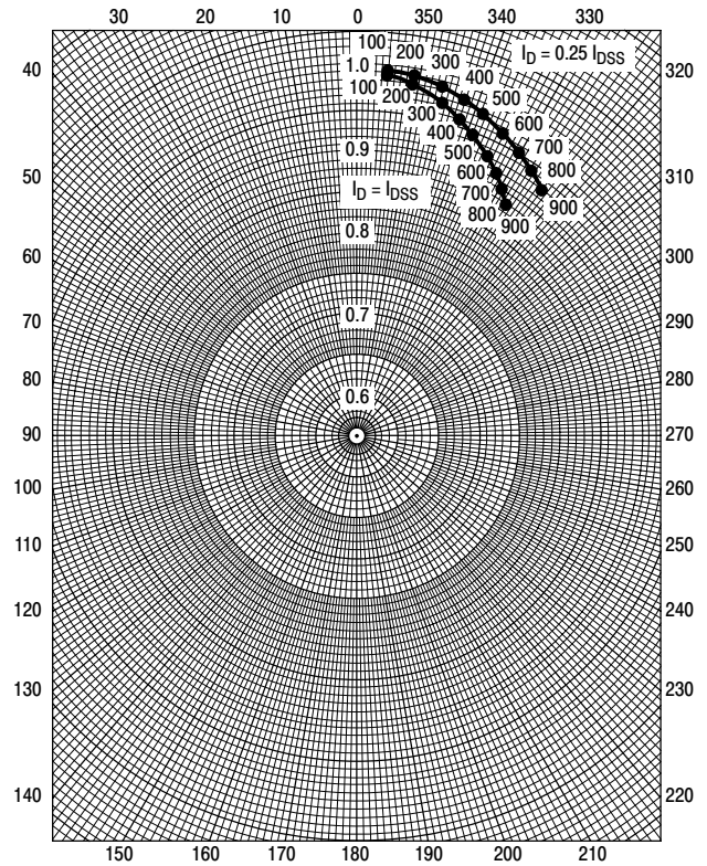
Figure 8. S_{22s}
