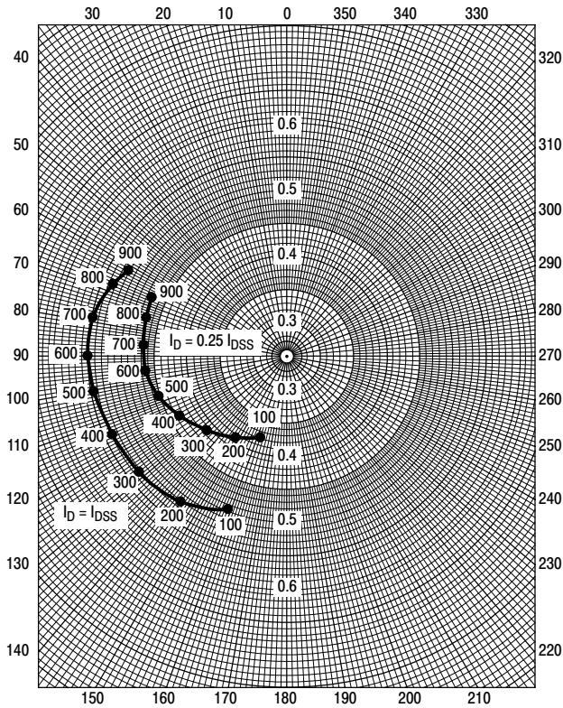
Figure 7. S_{21s}
