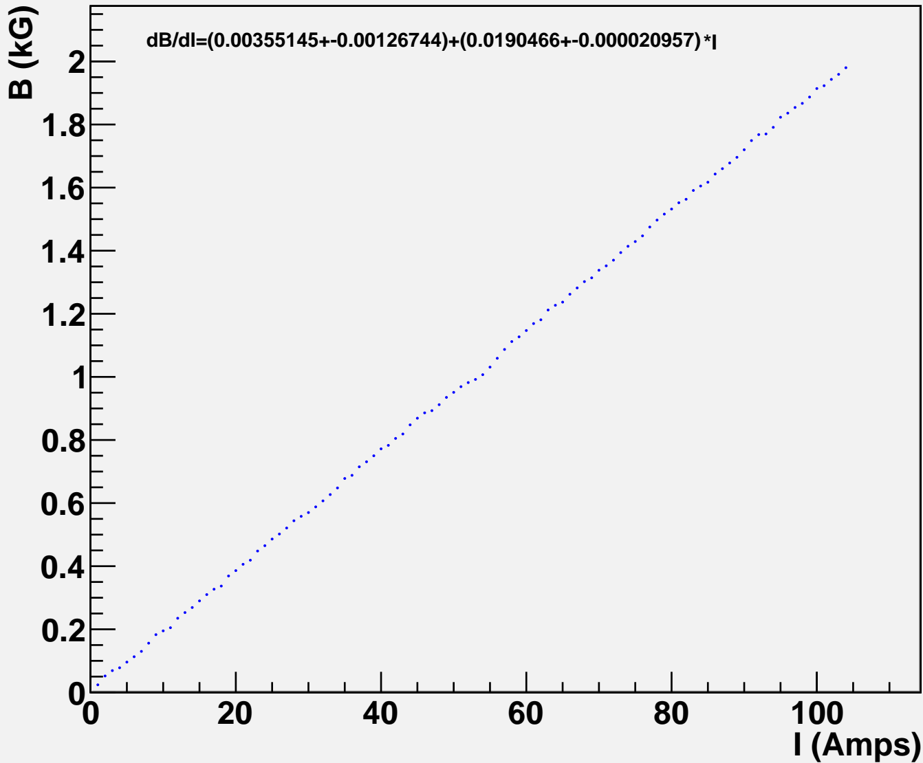
Type 2 Quad: Magnetic field as a function of current dB/dI
