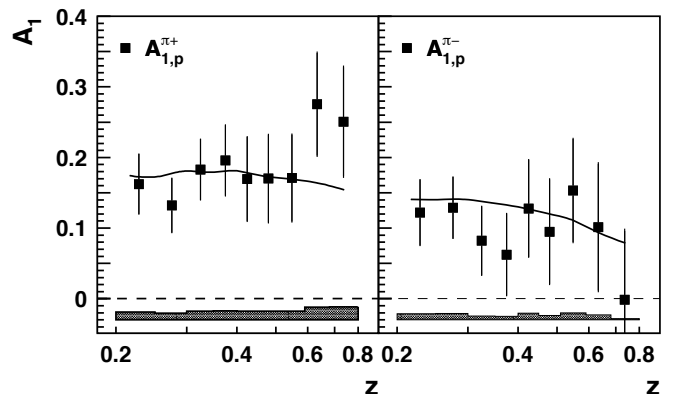
FIG. 15: The semi-inclusive Born asymmetries for positive and negative pion production on the proton as a function of z . The error bars indicate the statistical uncertainties and the error band represents the systematic uncertainties. The solid line is the z dependence from the Monte Carlo simulation of the asymmetries.
