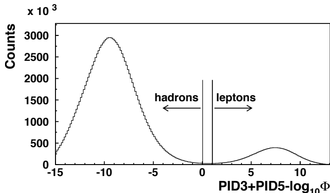
FIG. 8: The distribution of the total PID value. This logarithmic ratio of probabilities includes the particle fluxes and the responses of all PID detectors. The left hand peak is the hadron peak, while the right hand peak originates from leptons. The limits that were applied in the analysis are shown as vertical lines.
