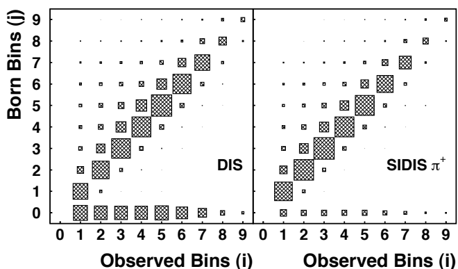
FIG. 24: Matrices n_u(i, j) = n_{\Leftarrow}(i, j) + n_{\Rightarrow}(i, j) for DIS events and SIDIS \pi^+ events on the proton. The binning shown corresponds to the 9 bins in x that were used in the asymmetry and \Delta q analysis (Tab. V). See the text for details.
