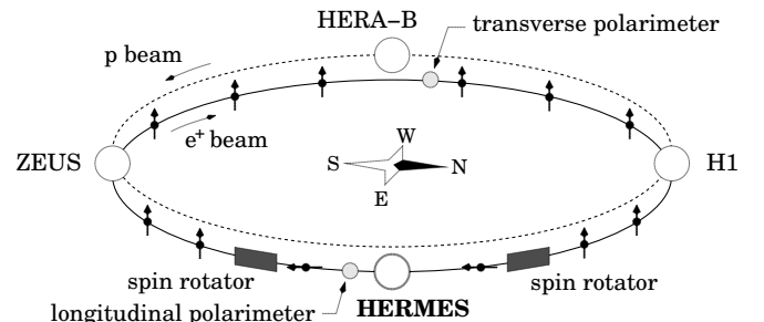
FIG. 2: Schematic diagram of the HERA accelerator layout until 2000 with the location of the four experiments. Also shown are the locations of the spin-rotators and the two polarimeters.
