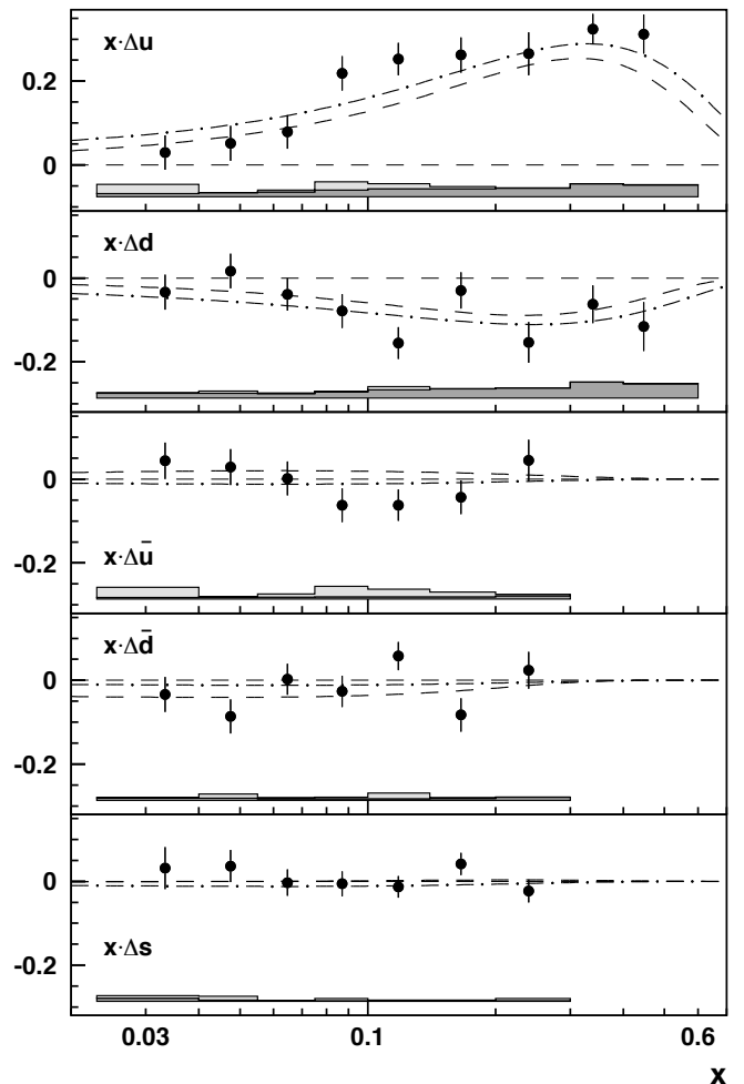
FIG. 20: The quark helicity distributions x \Delta q(x, Q_0^2) evaluated at a common value of Q_0^2 = 2.5 \text{ GeV}^2 as a function of x . The dashed line is the GRSV2000 parameterization (LO, valence scenario) [18] scaled with 1/(1 + R) and the dash-dotted line is the Blümlein-Böttcher (BB) parameterization (LO, scenario 1) [66]. See Fig. 19 for explanations of the uncertainties shown.
