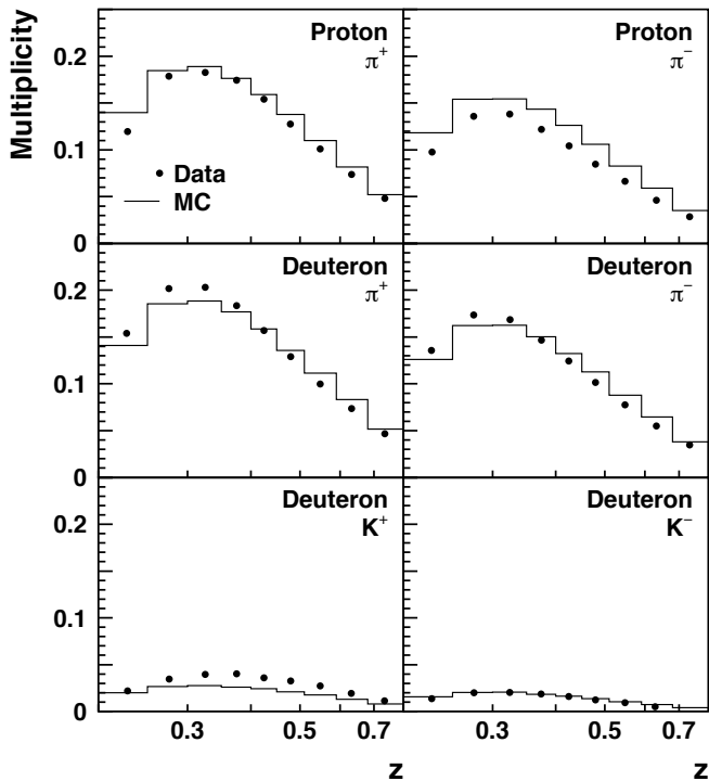
FIG. 17: Multiplicities of charged pions and kaons in the HERMES acceptance compared with Monte Carlo data as function of z . Statistical uncertainties in the data are too small to be visible. The multiplicities shown were not corrected for radiative and instrumental effects.
