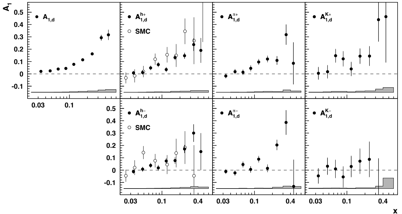
FIG. 14: The inclusive and semi-inclusive Born level asymmetries on the deuteron. One data point at x = 0.45 for the K^- asymmetry including its large error bar is outside the displayed range; all data points are listed in Tab. XIII. See Fig. 13 for details.
