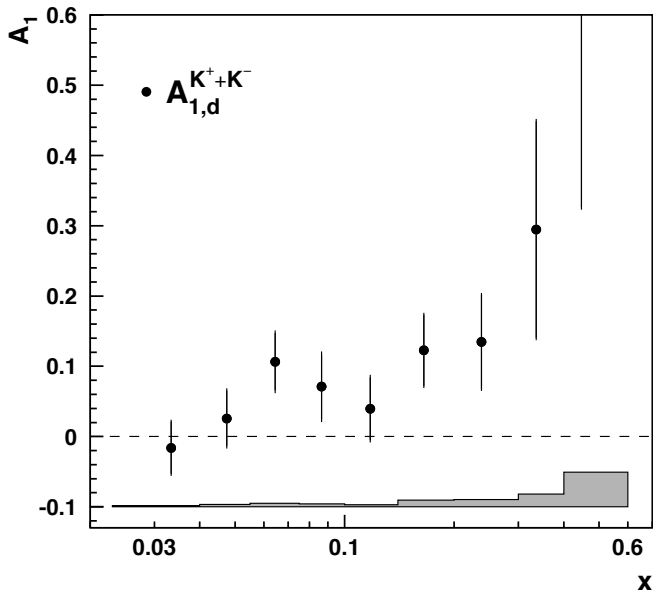
FIG. 22: The semi-inclusive Born level asymmetry A_{1,d}^{K^+K^-} for the total charged kaon flux on a deuterium target, corrected for instrumental smearing and QED radiative effects. The uncertainties are presented analogously to Fig. 13.
