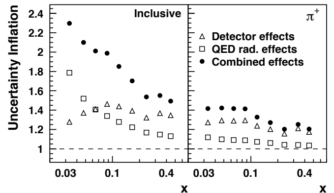
FIG. 12: Uncertainty inflation caused by detector smearing and QED radiative effects. The left hand panel shows the uncertainty inflation of the inclusive asymmetry for the proton and the right hand panel that of the positive pion asymmetry. In both panels the open triangles present the uncertainty inflation caused by detector effects, the open squares present the inflation caused by QED radiative effects, and the filled circles show the total uncertainty inflation.
