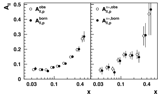
FIG. 11: The observed asymmetries A_{\parallel} and A_{\parallel}^{\pi^+} on the proton target compared with the corresponding Born asymmetries. The Born asymmetries are offset horizontally for better presentation. See the text for details.
