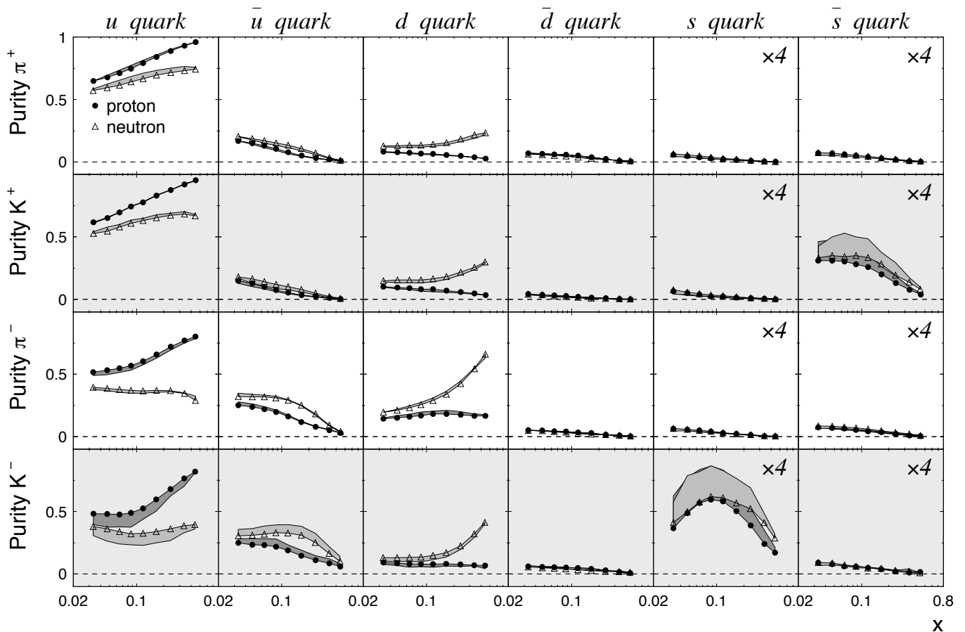
FIG. 18: Purities for positive and negative pions and kaons on a proton and a free neutron target. Each column corresponds to scattering off a certain quark flavor. The shaded bands indicate the estimated systematic uncertainties due to the fragmentation parameters. The estimate derives from a comparison of two parameter sets. See text for details.
