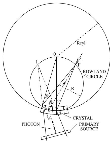
Figure 1: Concept of the monochromatic source.
