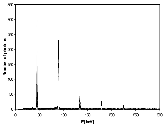
Figure 3: Typical spectrum from a symmetrically-cut crystal
