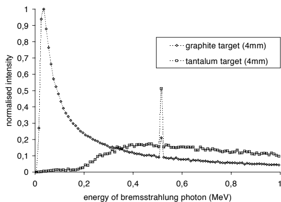
Figure 2: Bremsstrahlung spectrum on the effective crystal surface for a graphite and a tantalum target
