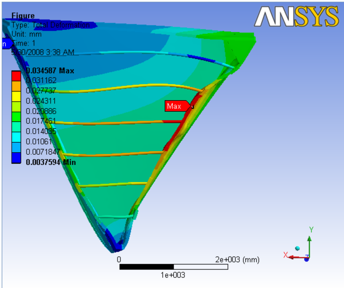
FIGURE 11 sector 1, Case 6 > Static Structural > Solution > X - Directional Deformation > Figure
