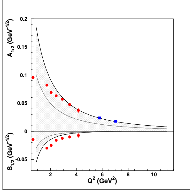
Figure 2: Transition \gamma_v N-N^*(1535) amplitudes based on LCSR, that utilized preliminary LQCD results of Distribution Amplitudes [19] in comparison with the data. CLAS data [115] are shown in red, while preliminary data on (A_{1/2}^2 + \epsilon S_{1/2}^2)^{1/2} combination of transition amplitudes at high Q^2 are shown in blue.
