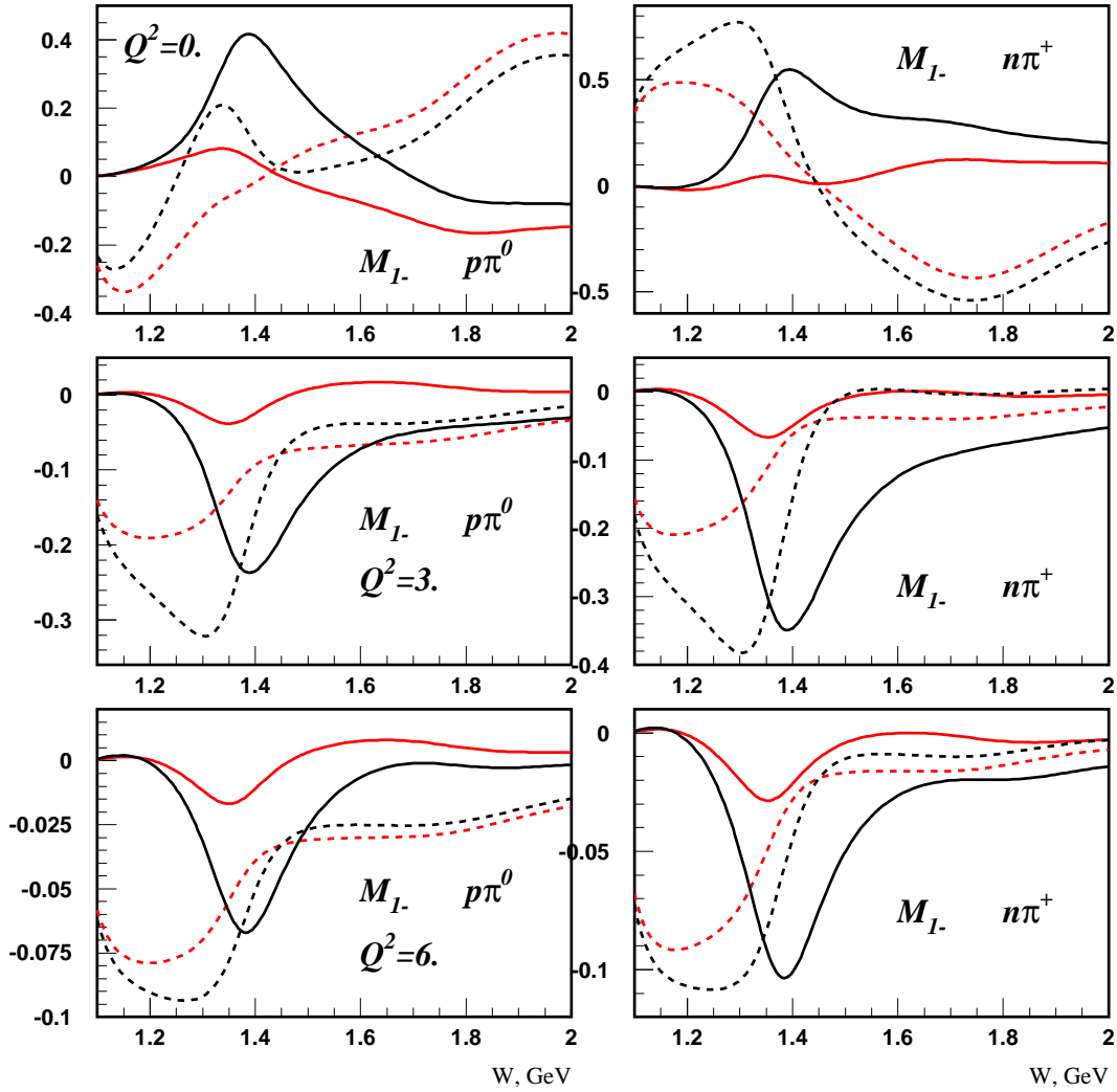
Figure 10: The M_{1-} multipole amplitude for the reactions \gamma^* p \rightarrow p\pi^0 (left) and n\pi^+ (right) at Q^2 = 0, 3, and 6 \text{GeV}^2 . Black curves are the total amplitudes, red curves represent the background; each separated into imaginary (real) part and represented by solid (dashed) curves.
