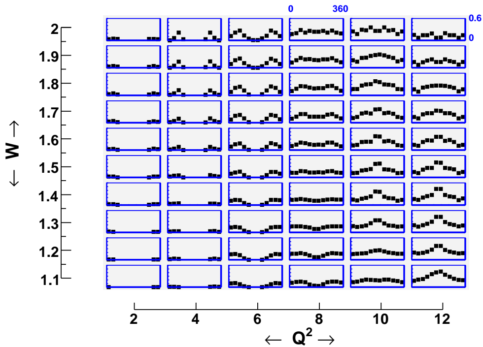
Figure 36: \phi_\pi evolution of the \pi^0 acceptance in the forward \cos\theta_\pi = 0.1 \pm 0.1 bin for the resonance region and the proposed Q^2 range.
