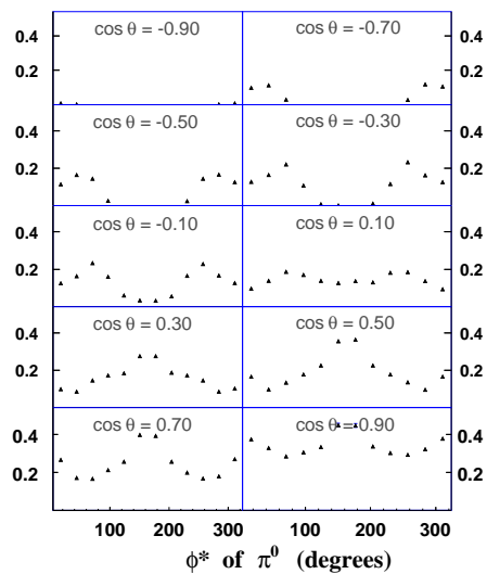
Figure 37: \phi_\pi evolution of the \pi^0 acceptance in a specific W and Q^2 bin for the full \cos\theta_\pi range.
