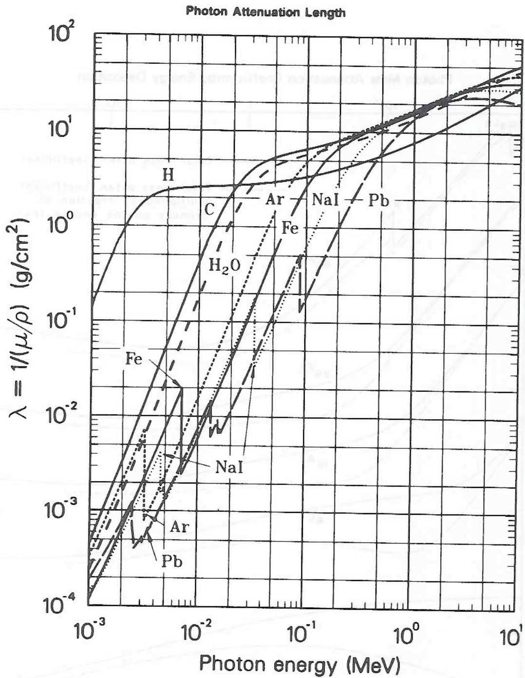
The photon mass attenuation length \lambda = 1 / (\mu / \rho) (also known as the mean free path) for various absorbers as a function of photon energy, where \mu is the mass attenuation coefficient.
