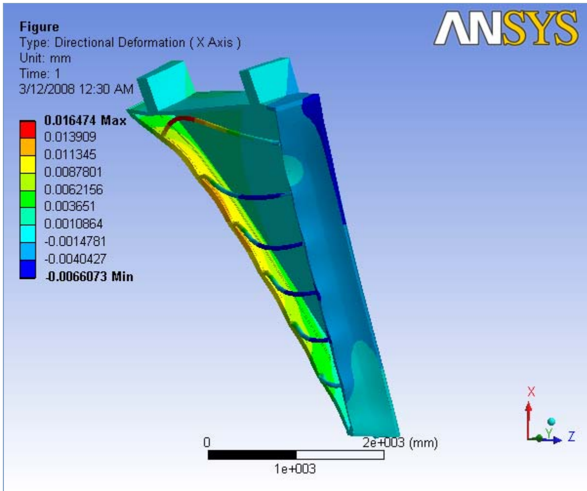
FIGURE 9 Model > Static Structural > Solution > y Directional Deformation > Figure
