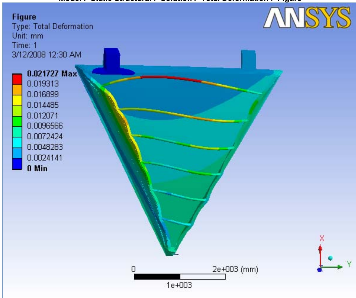
FIGURE 7 Model > Static Structural > Solution > Total Deformation > Figure
