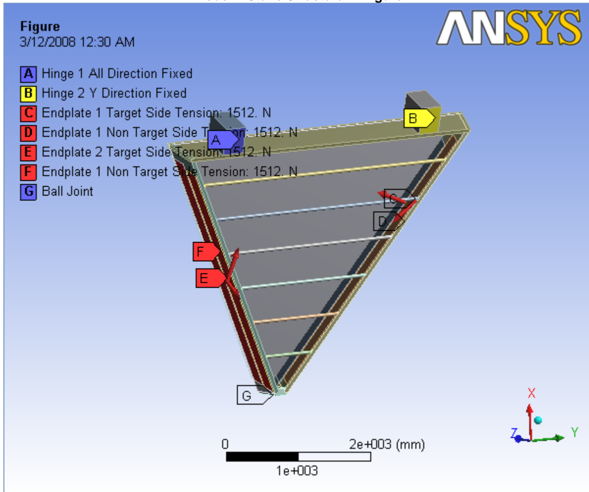
FIGURE 1 Model > Static Structural > Figure
