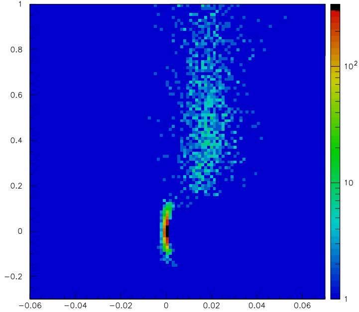
Figure 21: Separation of 2\pi events from the multi-pion background, using the missing energy - M_{p\pi+\pi^-X}^2 kinematic correlation, with 2\pi events in the spot around zero and 3 pion events in the vertical strip.
