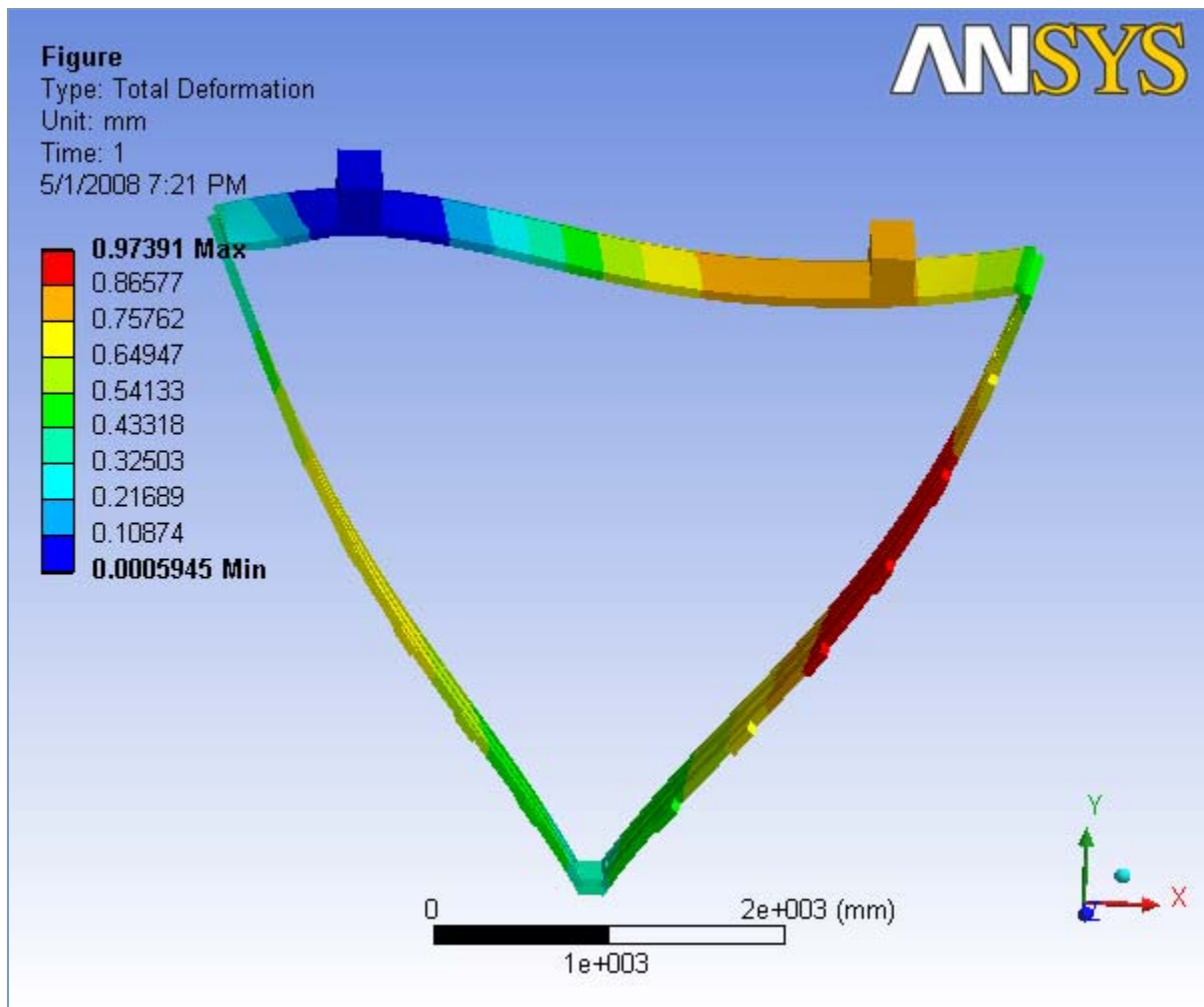
FIGURE 11 Ideal Slice with Gravity (No Hexcel, No rods, No Wire Tensions) > Static Structural > Solution > X Deformation > Figure
