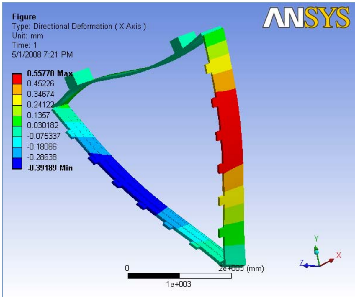
FIGURE 12 Ideal Slice with Gravity (No Hexcel, No rods, No Wire Tensions) > Static Structural > Solution > Y Deformation > Figure
