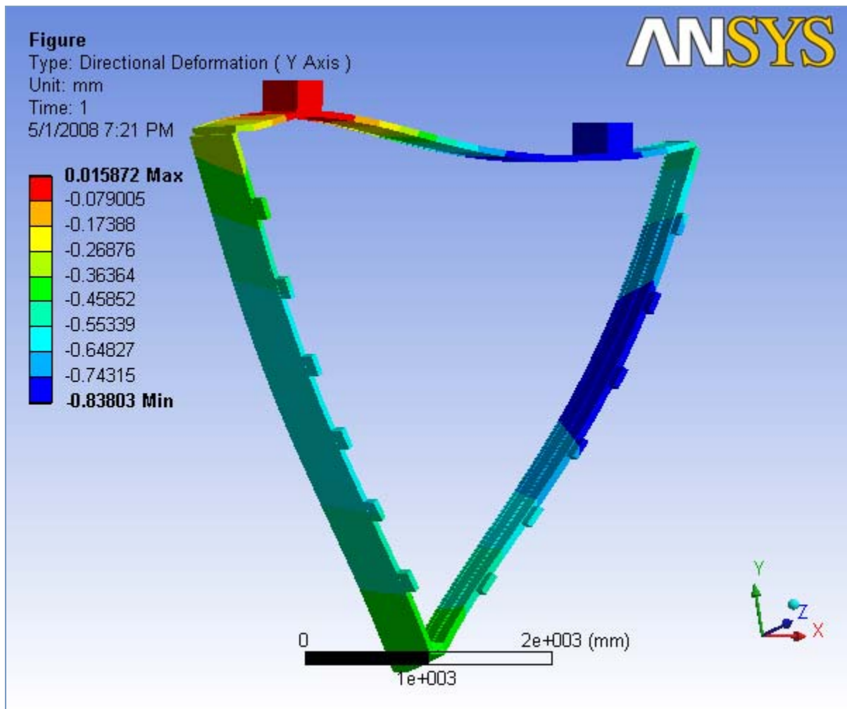
FIGURE 13 Ideal Slice with Gravity (No Hexcel, No rods, No Wire Tensions) > Static Structural > Solution > Z Deformation > Figure
