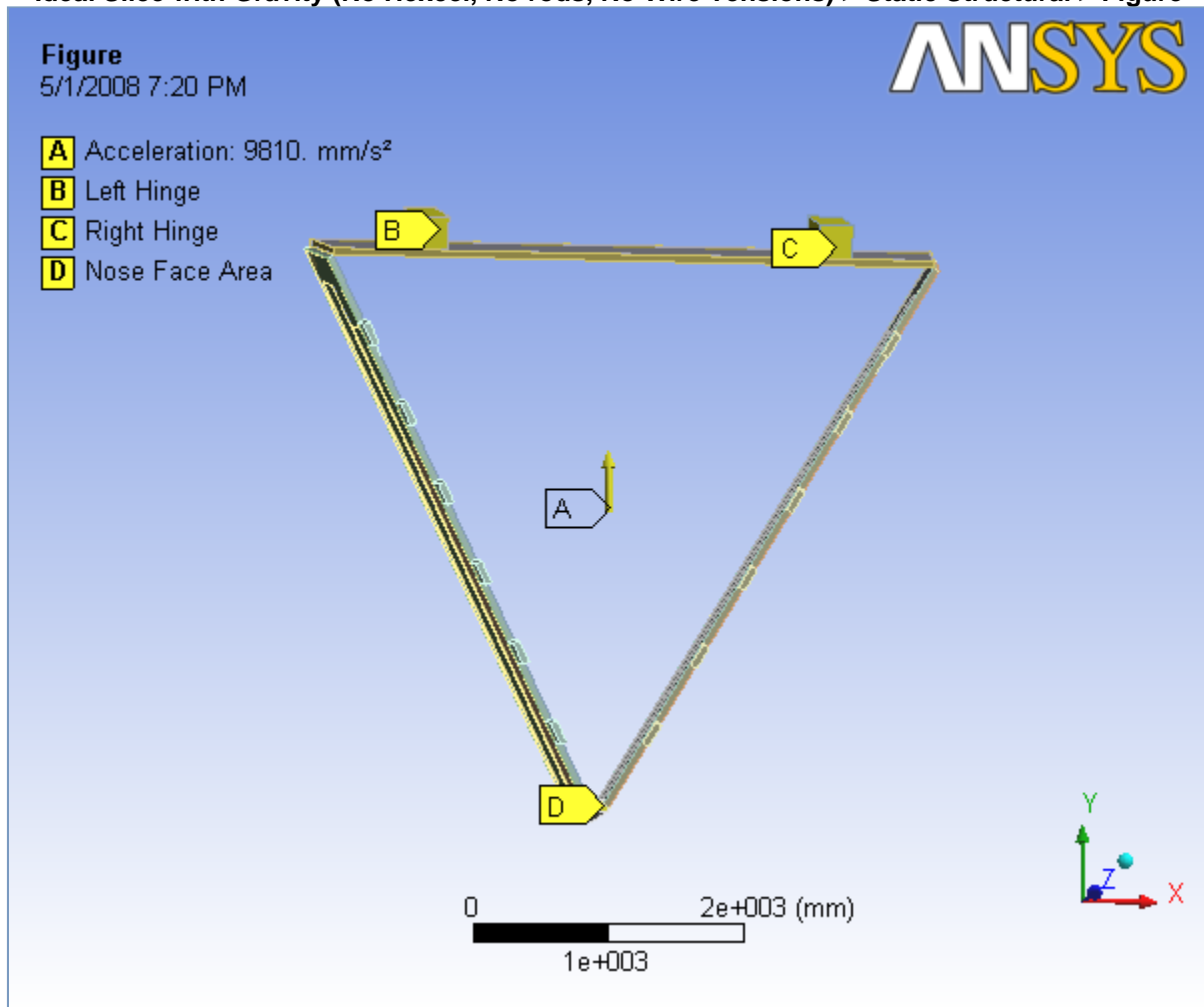
FIGURE 1 Ideal Slice with Gravity (No Hexcel, No rods, No Wire Tensions) > Static Structural > Figure
