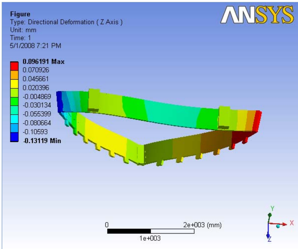
FIGURE 14 Ideal Slice with Gravity (No Hexcel, No rods, No Wire Tensions) > Static Structural > Solution > Equivalent Stress > Figure
