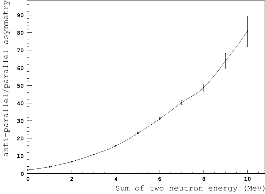
Figure 4.3: Calculated 2n asymmetry (antiparallel/parallel) as a function of the sum of two neutron energies
