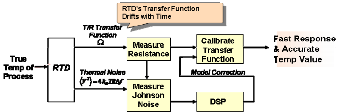
Figure 3. Johnson noise thermometry measurement process block diagram.
