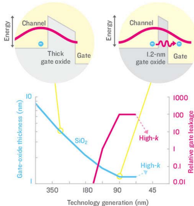
Figure 10. Gate leakage has increased 100-fold in the last three generations of transistors (© 2009 IEEE).
