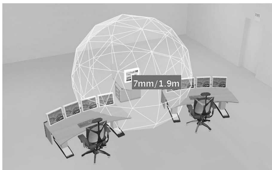
Figure 23. Evaluation of label legibility showing the height of the text and calculated range of legibility (Copyright_Feb. 2009 by the American Nuclear Society, La Grange Park, Illinois). 118
