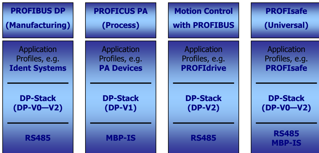
Figure 6. Application-oriented features of PROFIBUS.
