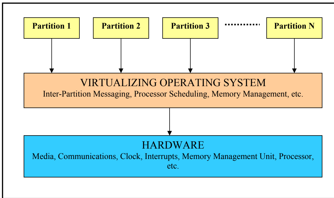
Figure 13. A simple model of an ARINC 653 partitioned system.
