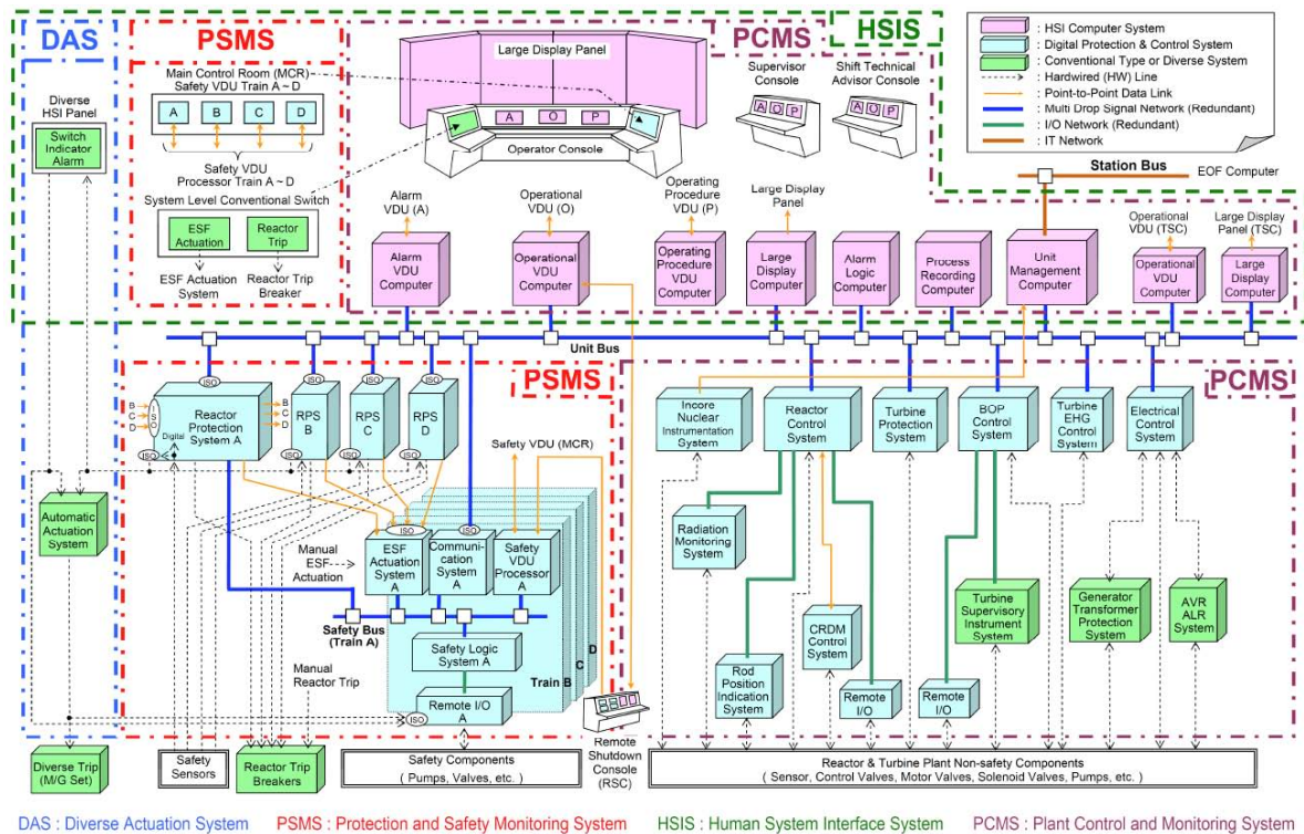
Figure 30. Overall architecture of the Advanced Pressurized-Water Reactor instrumentation and controls system.
