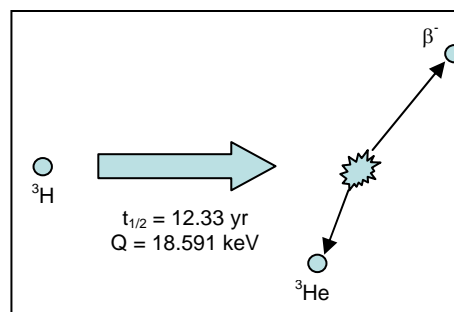
Figure 16: Virtually all helium-3 in present worldwide stores has been produced as a product of tritium \beta -decay.
