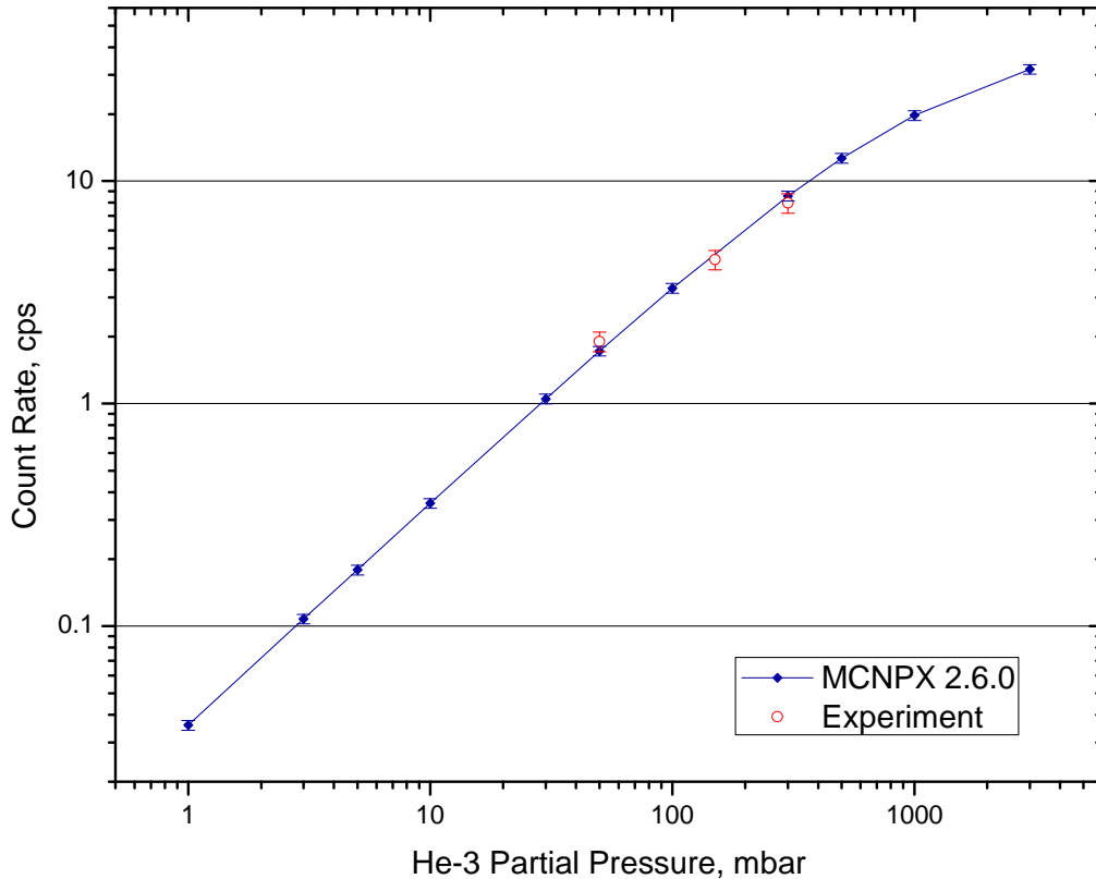
Figure 25: Results of the He-3 partial-pressure experiment
