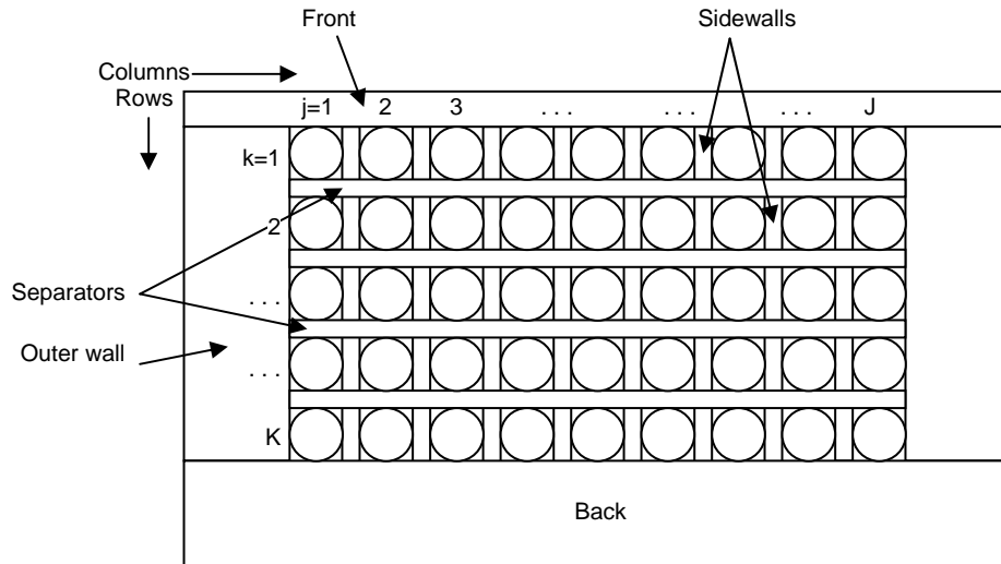
Figure 31: Diagram of an ANDY-type detector, specifying all parameters to be optimized.
