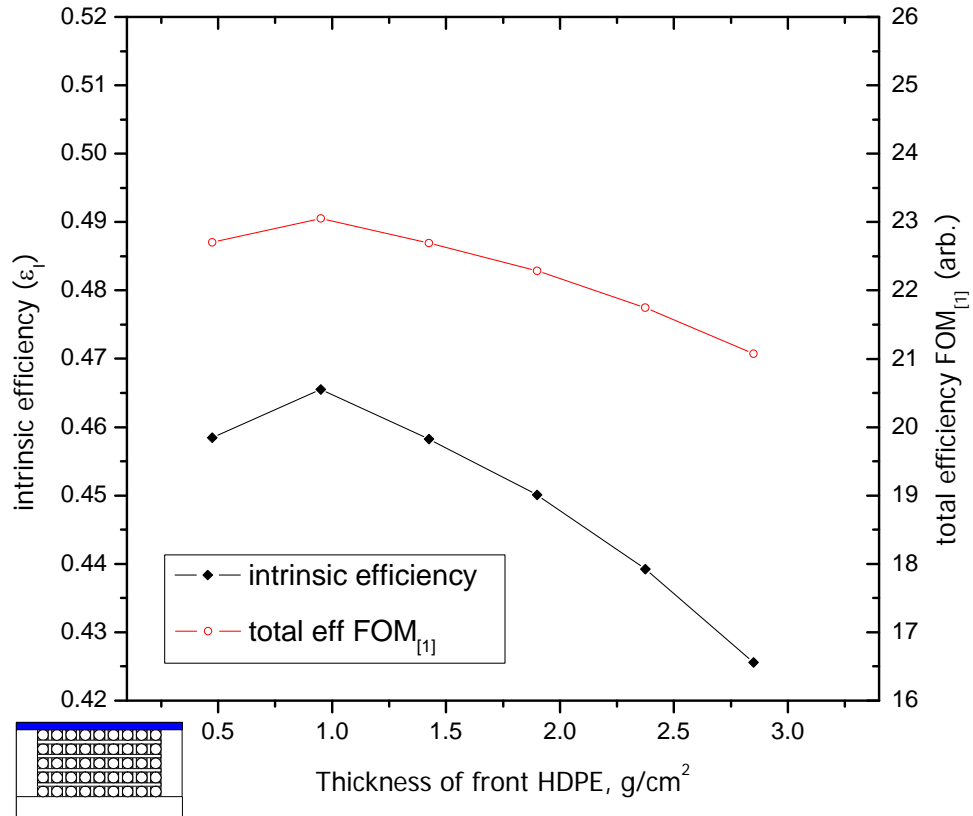
Figure 34: Efficiency parameters vs. front face-thickness for the semi-infinite ANDY array. The surface area is constant throughout this comparison, and the two curves are identical in shape. The statistical error bars are less than 1%.
