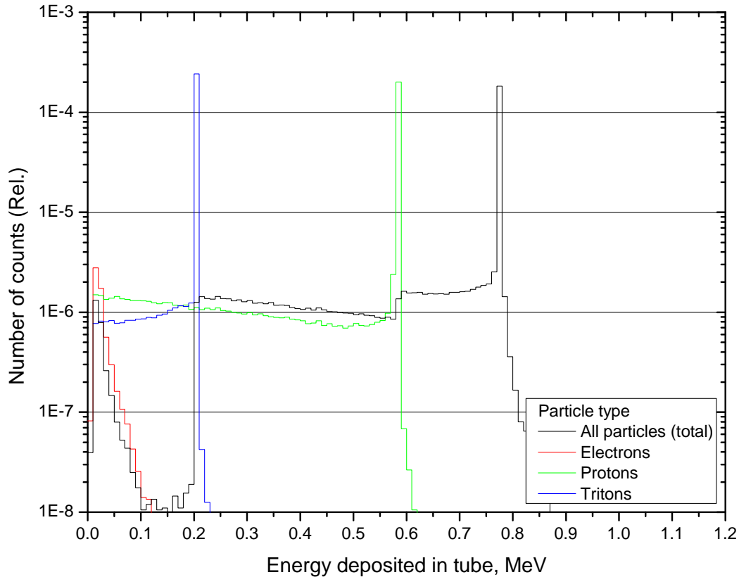
Figure 23: MCNPX pulse-height light tally of energy deposited in He-3 tube from 3\text{He}(n,p)3\text{H} reactions, broken down by particle type 22 . The steps in the sum spectrum correspond to wall effects (see § 1.2.1.2). Notice that the peak in the proton spectrum is slightly shorter than that for the tritons; this demonstrates that more protons stop in the wall because of their greater range. An energy threshold of 191 keV was used to identify pulses produced by neutron capture events.
