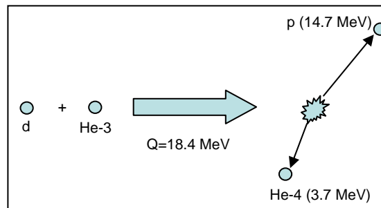
Figure 15: The d-He3 fusion reaction
