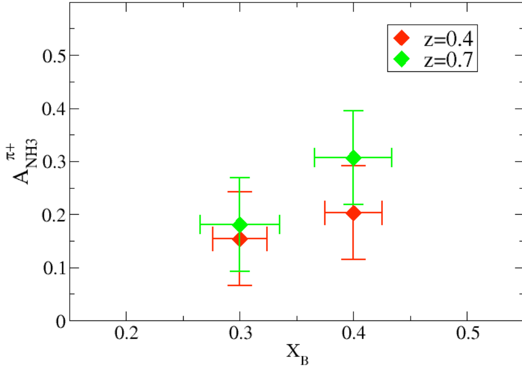
Fig. 3.20: x_B versus A_{NH3}^{\pi^+} SIDIS Asymmetry.
