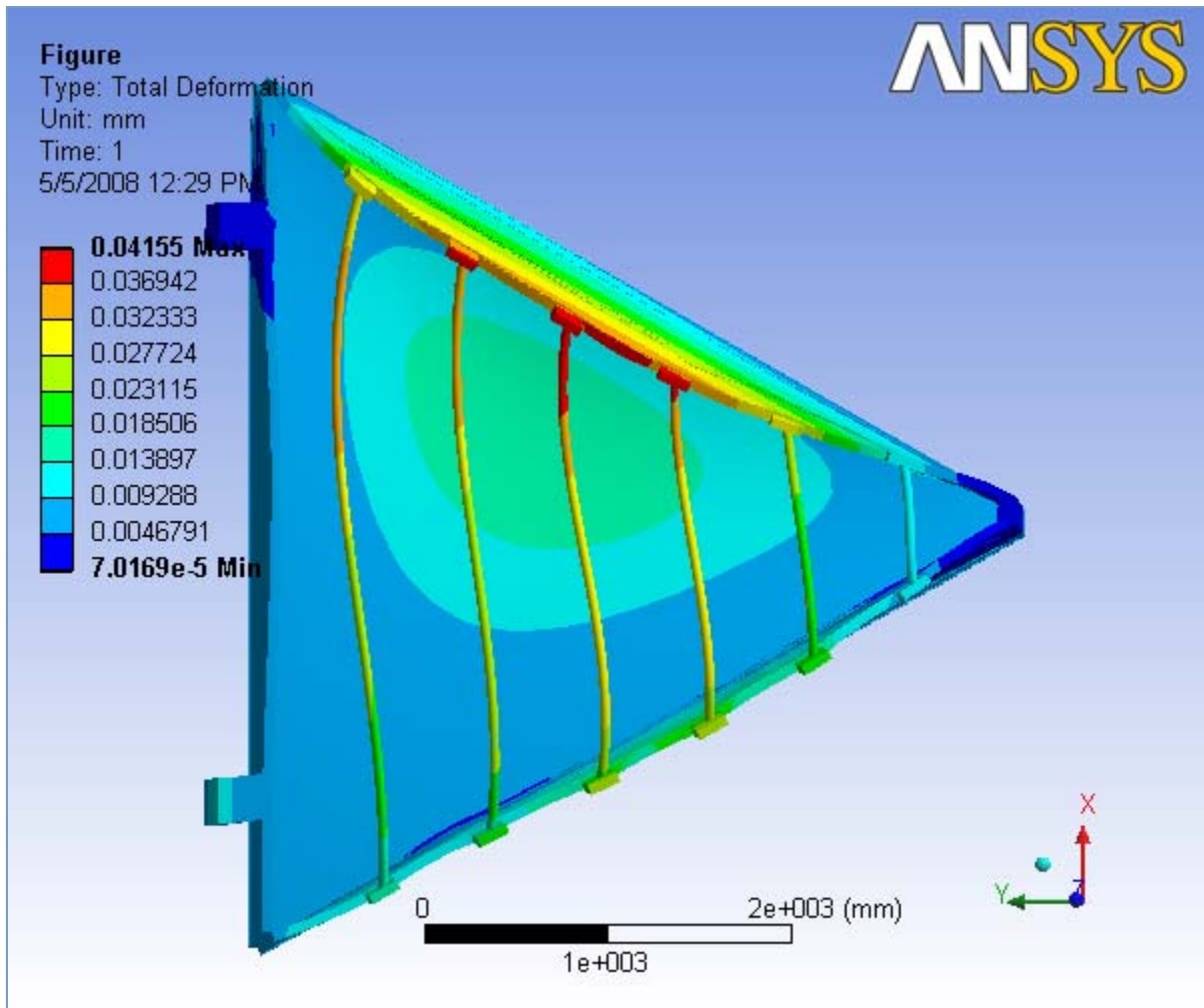
FIGURE 11 Orientation 1.1 > Static Structural > Solution > X - Directional Deformation > Figure
