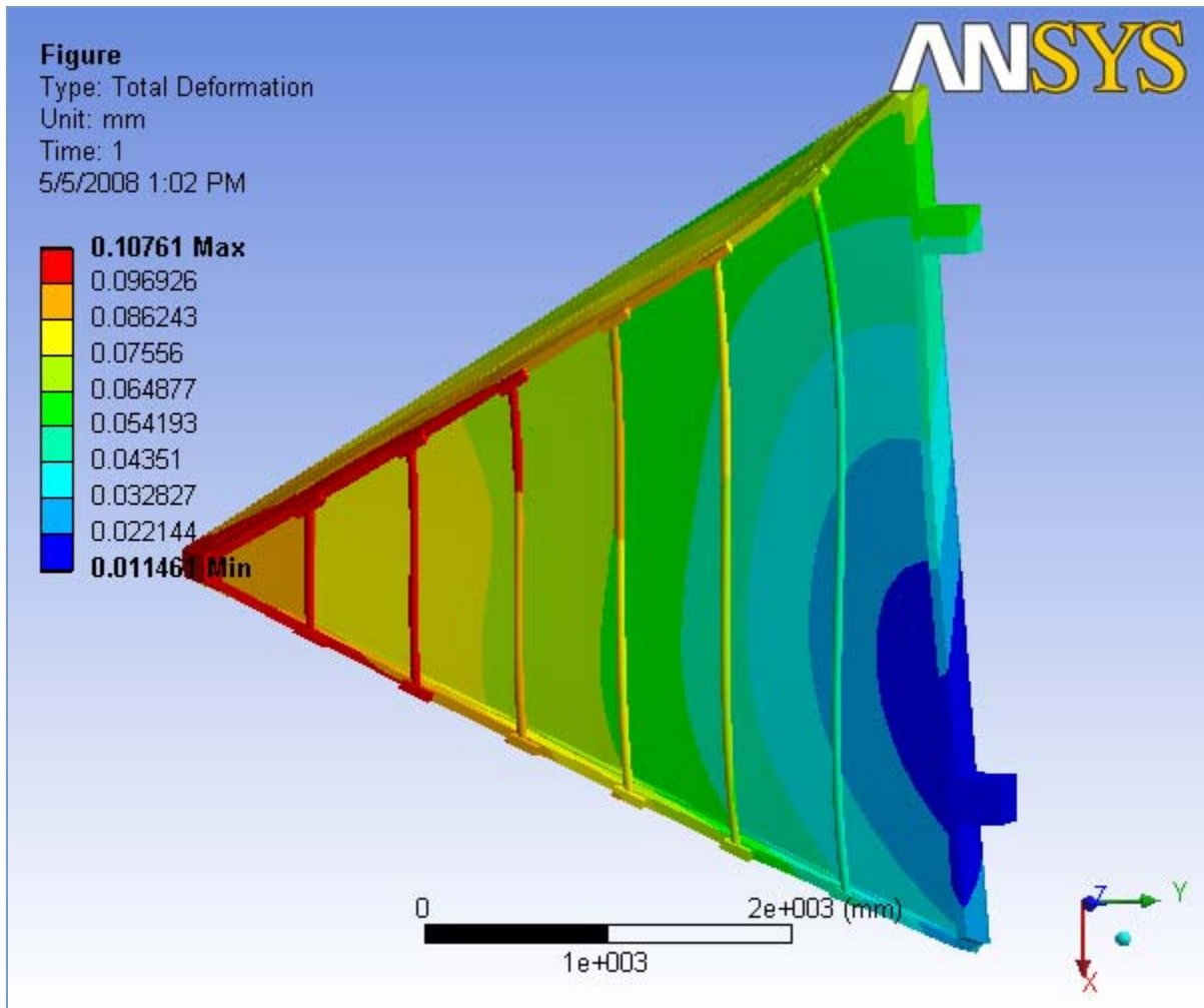
FIGURE 11 Orientation 4.1 > Static Structural > Solution > X - Directional Deformation > Figure
