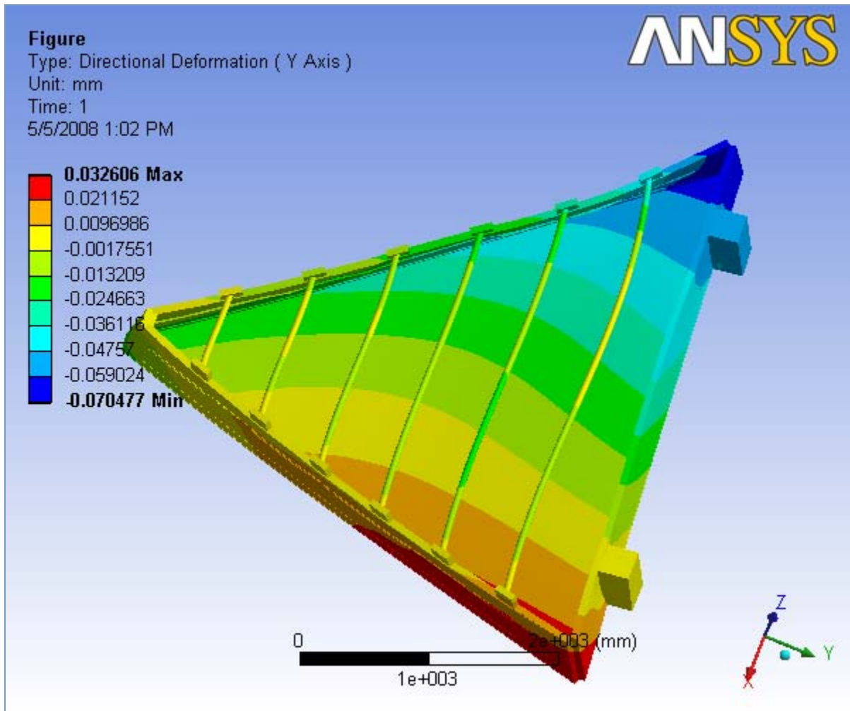
FIGURE 13 Orientation 4.1 > Static Structural > Solution > Z - Directional Deformation > Figure
