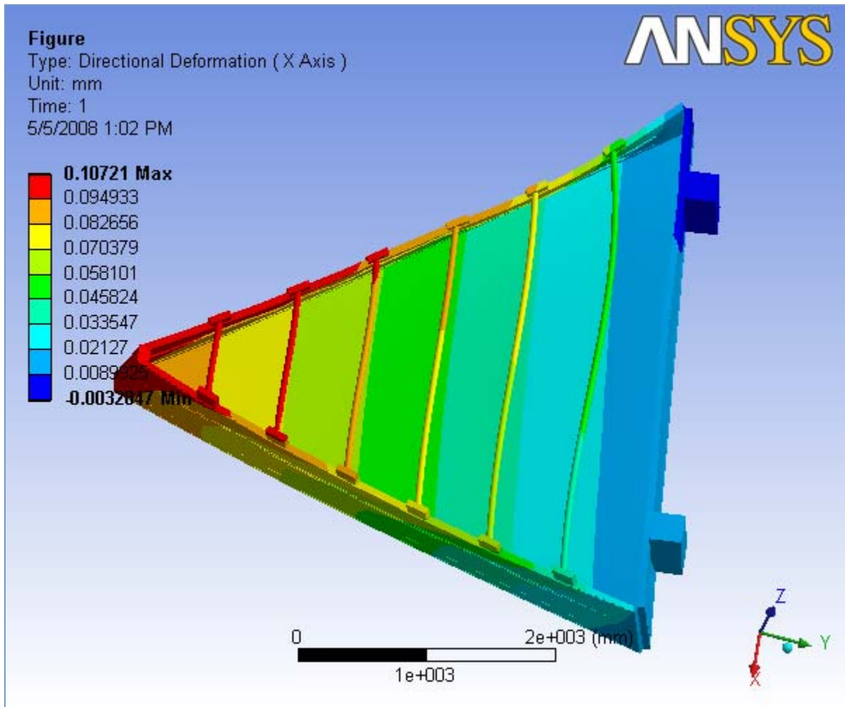
FIGURE 12 Orientation 4.1 > Static Structural > Solution > Y - Directional Deformation > Figure
