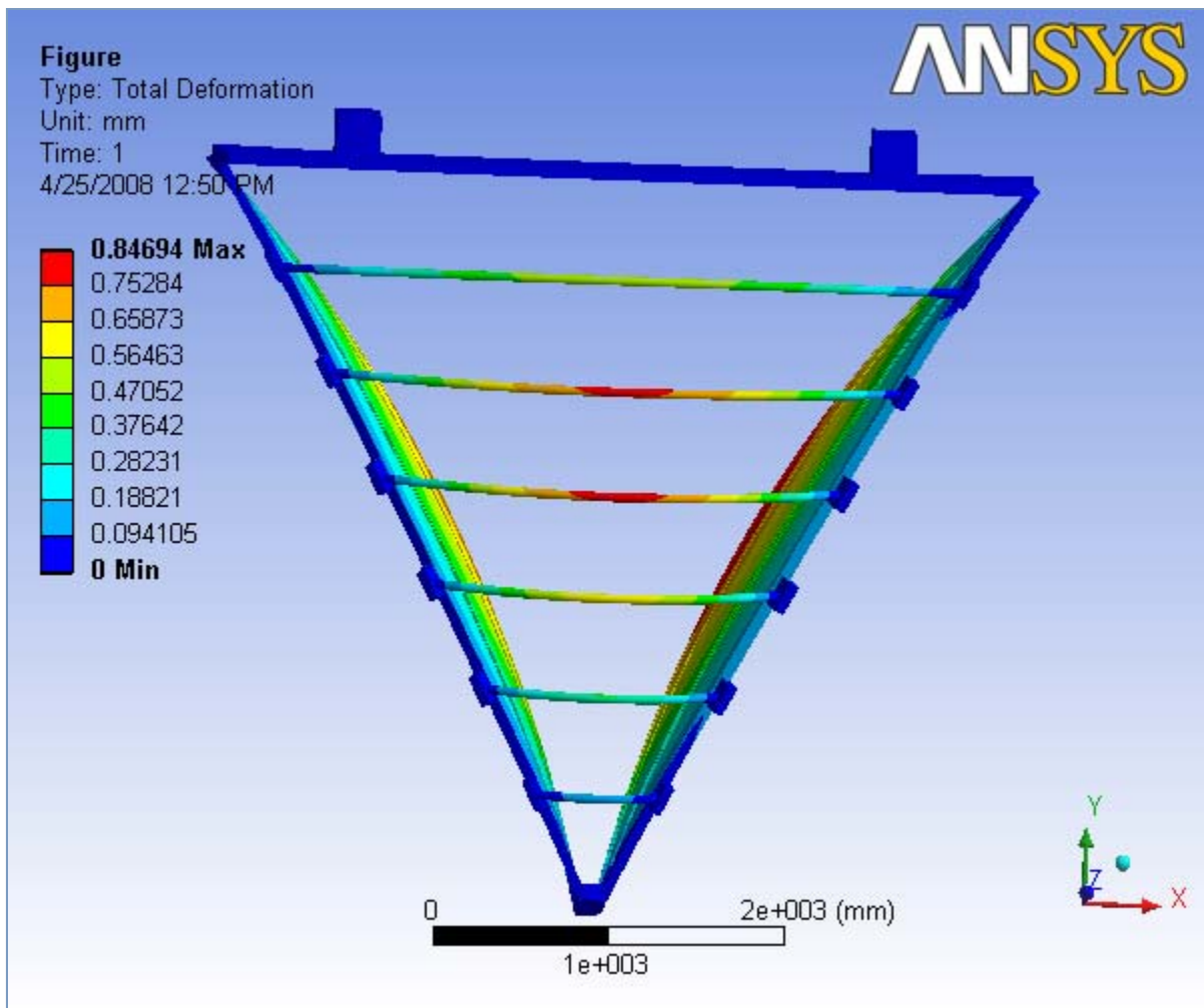
FIGURE 9 Model > Static Structural > Solution > X Deformation > Figure
