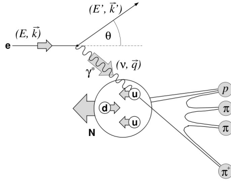
Figure 1. Diagram of The Semi Inclusive Deep Inelastic Scattering [7] .
