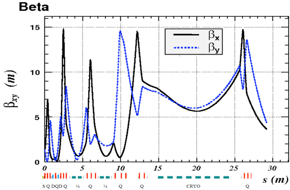
FIG. 68: The twiss \beta_{xy} functions of the positron beam as a function of the central orbit are plotted in Two-Dipole configuration. The solid line is \beta_x and dashed line is \beta_y . The boxes under the horizontal axis show the location of the magnets, where the solenoid (S), dipoles (D), quadrupoles (Q), quarter cryomodules (1/4) and full cryomodule (CRYO).
