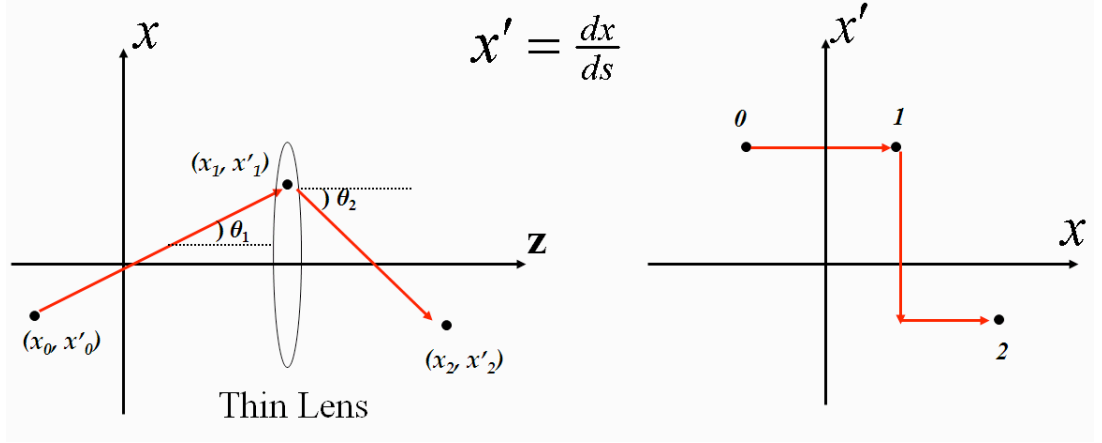
FIG. 3: On the left, a particle's movement is shown in the cartesian coordinate where x' = dx/ds is the slope of the particle which it makes in the horizontal plane. Here the particle has x_0 as the initial position traveling in a drift space with an angle \theta_1 , where at x_1 a thin quadrupole changes the angle to -\theta_2 . The particle's movement is illustrated in x - x' phase space on the right coordinate system.
