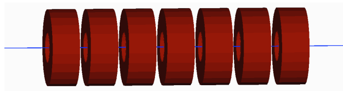
(c) C100 7-cell RF cavities are simulated with pillbox cavities in G4.
