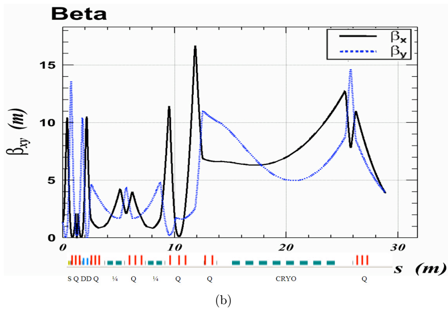
FIG. 81: (a) The 1\text{-}\sigma beam size of the positron beam as a function of the central orbit in the microtron dipole lattice is plotted. The solid line is \sigma_x and dashed line is \sigma_y . (b) The twiss \beta_{xy} functions for the same lattice are plotted where the solid line is \beta_x and dashed line is \beta_y . The boxes under the horizontal axis show the location of the magnets, where the solenoid (S), dipoles (D), quadrupoles (Q), quarter cryomodules (1/4) and full cryomodule (CRYO).
