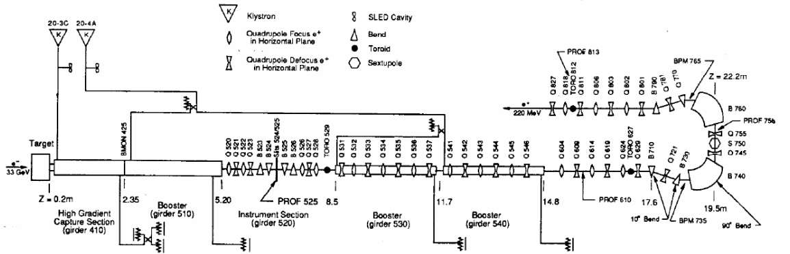
FIG. 19: The detailed drawing of the SLAC positron source, capture line, linac and 180^\circ positron return line [31]. The positron target is located on the left of the schematic, where electron beam is coming from left [28].
