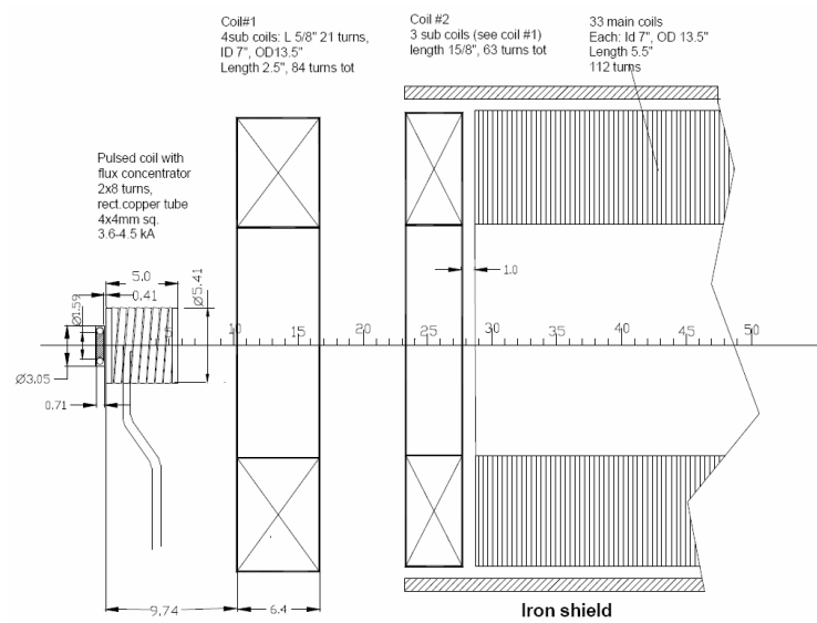
(a) Geometry of the positron capturing optics in CESR.
