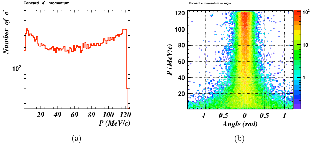
FIG. 85: (a) The momentum distribution of the electrons in the forward direction. Incident p(e^-)=126 MeV/c on a 2 mm tungsten. Forward direction means downstream of the tungsten converter. The momentum distribution shows a uniform distribution from 0 to 120 MeV. (b) The p - \theta distribution of the forward electrons. The 0-degree line from the target is dominated by high energy electrons ( \geq 60 MeV/c)
