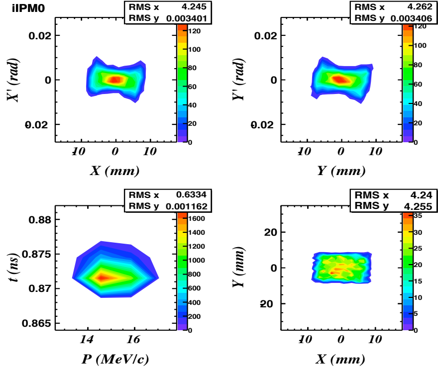
FIG. 73: Transverse and longitudinal phase space of the beam after the solenoid in Two-Dipole lattice. \varepsilon_x = 13.3 mm·mrad \varepsilon_y = 13.3 mm·mrad.
