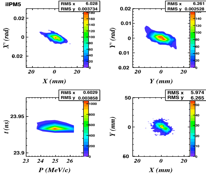
FIG. 76: (a) Transverse and longitudinal phase space of the beam right after the 1st quarter cryomodule in Two-Dipole lattice \varepsilon_x = 12 mm·mrad \varepsilon_y = 9 mm·mrad (b) Right before the 2nd quarter cryomodule \varepsilon_x = 10 mm·mrad \varepsilon_y = 8 mm·mrad.
