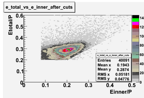
Figure 5. E_{total} vs E_{inner} after cuts were applied.
