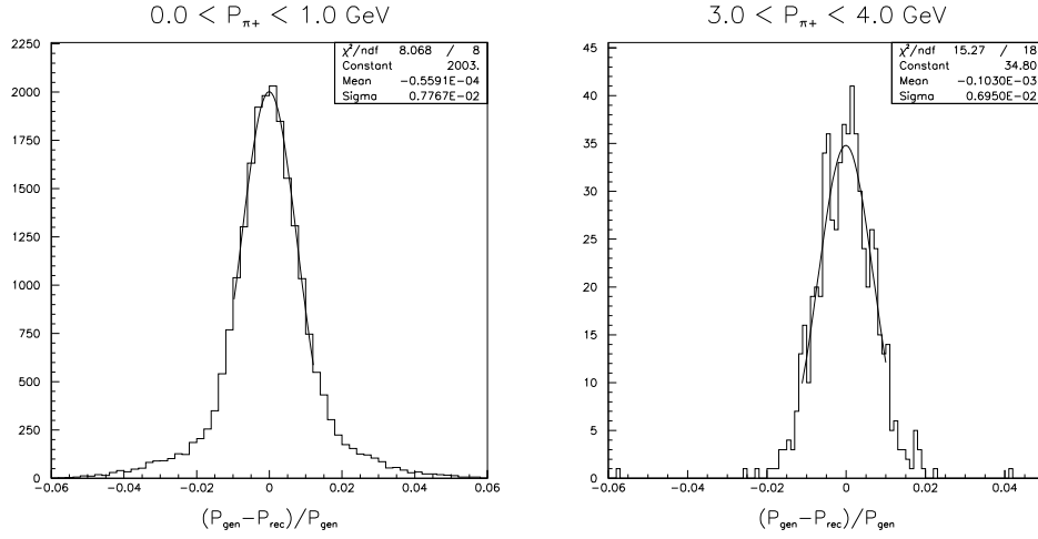
Figure 26: Momentum resolution for \pi^+ . p_{rec} and p_{gen} represent the momentum for reconstructed and generated particles, respectively.
