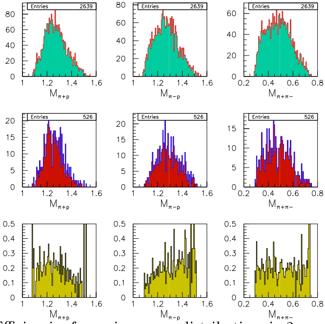
Figure 23: Efficiencies for various mass distributions in 2\pi production averaged over W from 1.5 to 1.7 GeV and Q^2 from 5.0 to 10.0 \text{GeV}^2 . The distributions for generated and accepted events are shown in the top and middle rows, respectively. The estimated efficiencies are presented in the bottom row.
