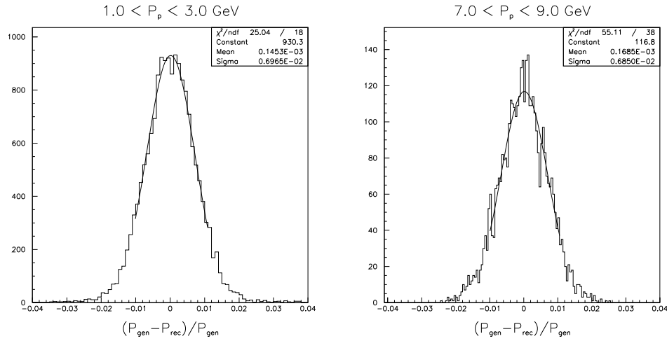
Figure 27: Momentum resolution for protons. p_{rec} and p_{gen} represent the momentum for the reconstructed and generated particles, respectively.
