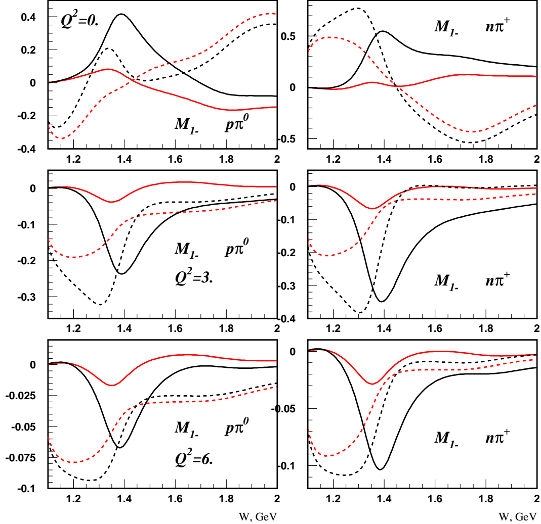
Figure 10: The M_{1-} multipole amplitude for the reactions \gamma^* p \rightarrow p\pi^0 (left) and n\pi^+ (right) at Q^2 = 0, 3, and 6 \text{ GeV}^2 . Black curves are the total amplitudes, red curves represent the background; each separated into imaginary (real) part and represented by solid (dashed) curves.
