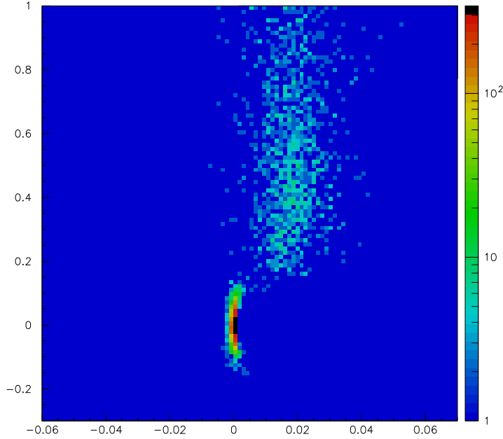
Figure 21: Separation of 2\pi events from the multi-pion background, using the missing energy - M_{p\pi+\pi-X}^2 kinematic correlation, with 2\pi events in the spot around zero and 3 pion events in the vertical strip.
