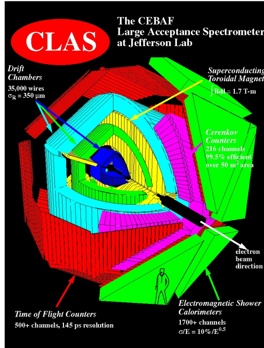
Figure 2. The CEBAF Large Acceptance Spectrometer at Jefferson Lab.
