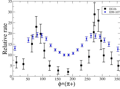
Figure 8. \varphi_{\pi^*} vs Relative rate for fixed \cos \theta_{\pi^+}^{CM} = 0.5 and W = 1.45 \text{ GeV} [19] , [20] .
